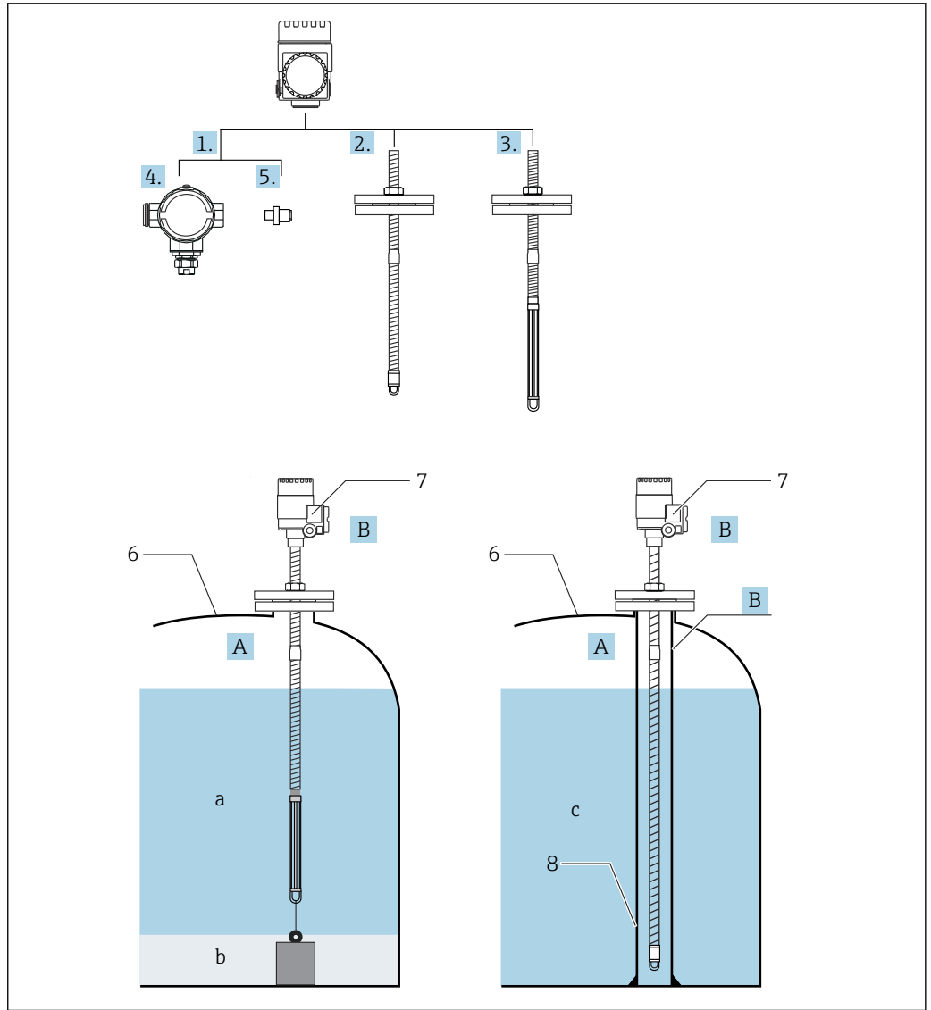
1 NMT539 installation
