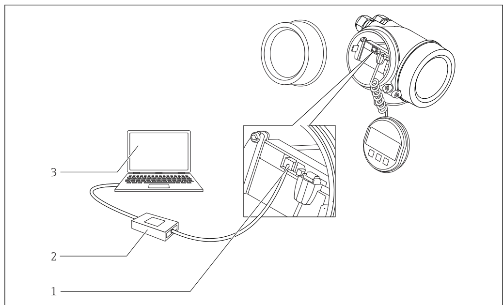
27 DeviceCare/FieldCare via interface service (CDI)
