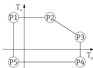
23 Aluminum housing, coated; process temperature -40 to +80 °C (-40 to +176 °F)
