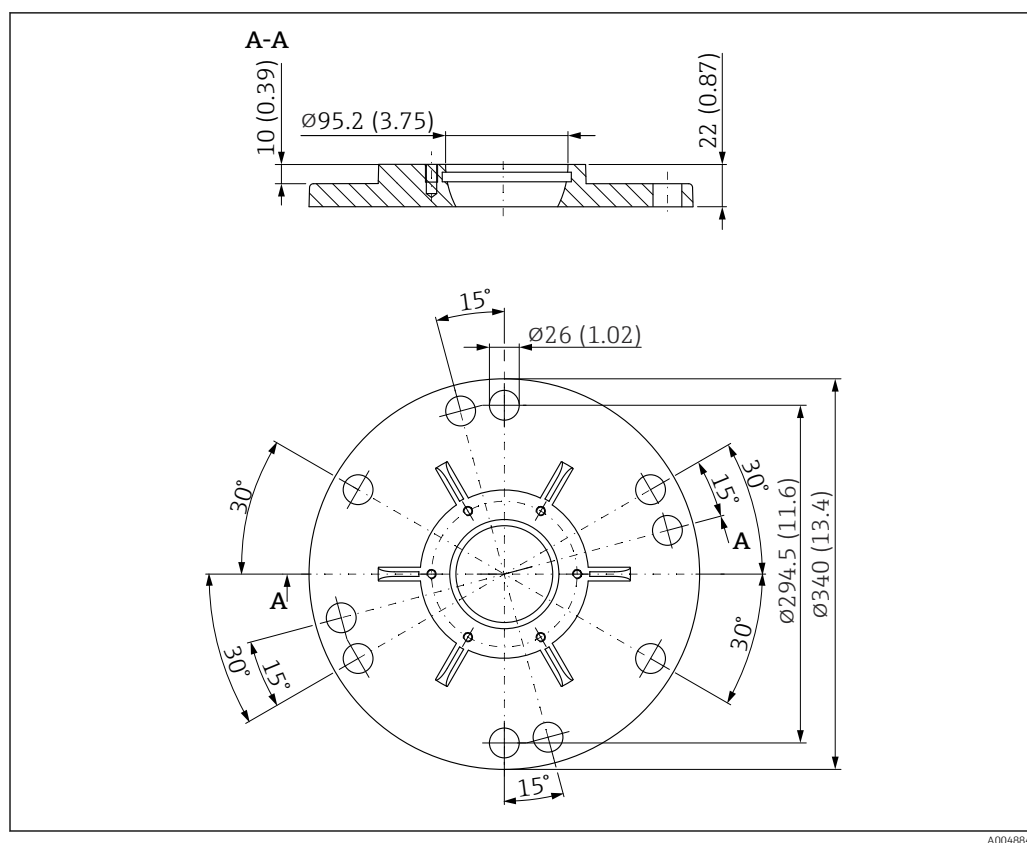
45 Dimensions of UNI flange 8"/DN200/200A for antennas with alignment unit. Unit of measurement mm (in)
