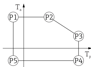
24 Aluminum housing, coated; process temperature -40 to +150 °C (-40 to +302 °F)
