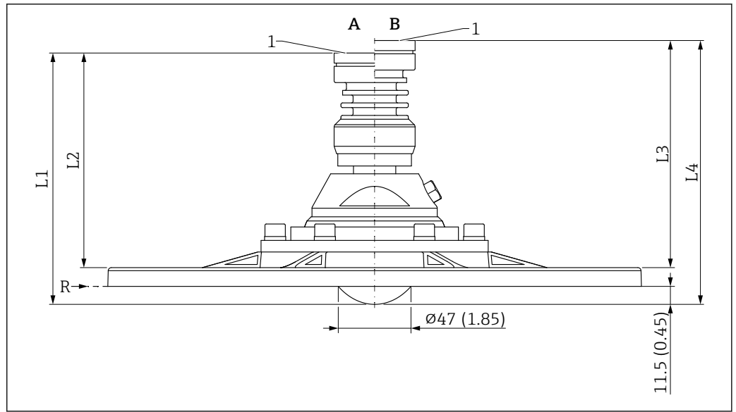
55 Dimensions of antenna flush mount, 80 mm (3 in), with UNI flange, alignment unit and purge air connection. Unit of measurement mm (in)
