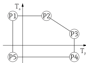
34 316L housing, hygiene; process temperature range: -40 to +150\text{ }^{\circ}\text{C} ( -40 to +302\text{ }^{\circ}\text{F} )
