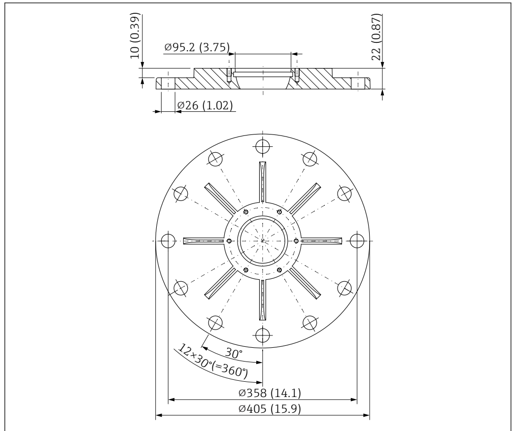
46 Dimensions of UNI flange 10"/DN250/250A for antennas with alignment unit. Unit of measurement mm (in)
