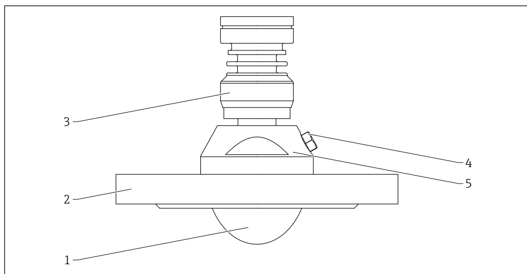
63 Material; antenna flush mount, 80 mm (3 in), with flange and purge air connection. Unit of measurement mm (in)
