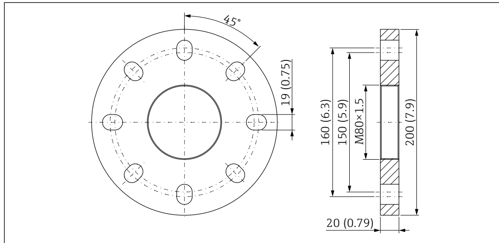
48 UNI flange 3"/DN80/80A for Drip-off antenna, PTFE, 50 mm (2 in) with purge air connection. Unit of measurement mm (in)
