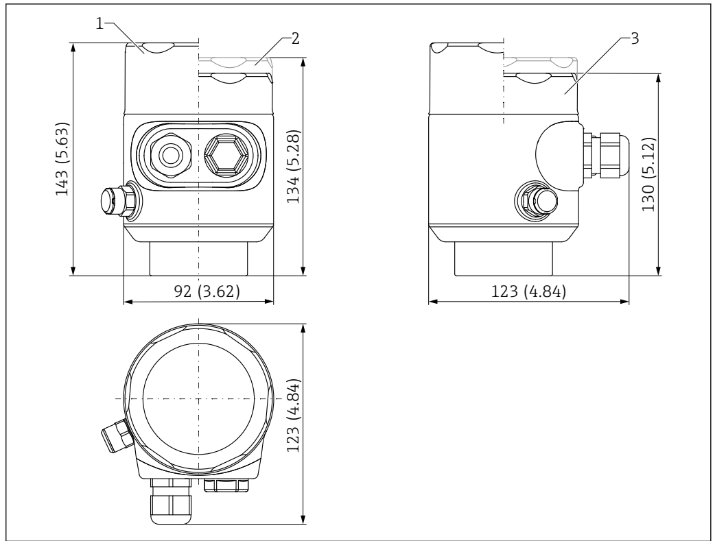
38 Dimensions of 316L single compartment housing, hygiene. Unit of measurement mm (in)
