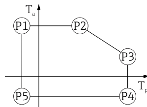
21 Plastic housing; process temperature -40 to +450 °C ( -40 to +842 °F)
