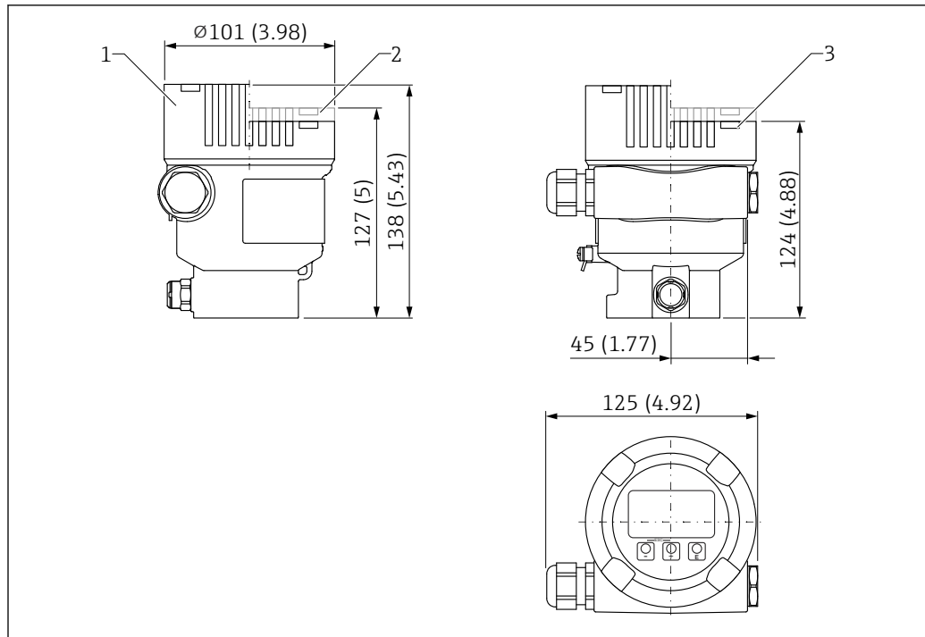
37 Dimensions of aluminum single compartment housing. Unit of measurement mm (in)
