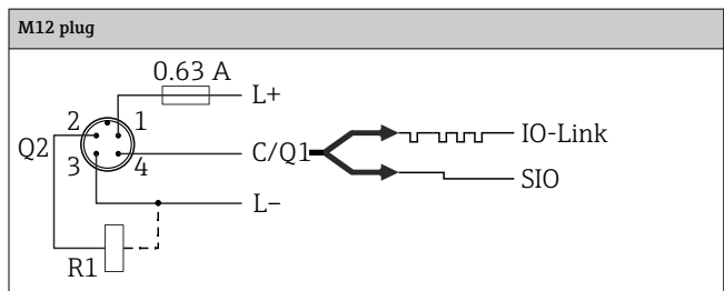
IO-Link: 2 x PNP switch output R1 and R2
