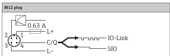
IO-Link: 1 x PNP switch output R1 with additional analog output 4 to 20 mA (active)
