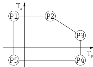
图 22 铝外壳, 带涂层; 过程温度范围: -40 \dots +200 \text{ }^{\circ}\text{C} ( -40 \dots +392 \text{ }^{\circ}\text{F} )
