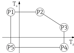
▣ 46 铝外壳, 带涂层; 过程温度范围: -20 ... +200 °C (-4 ... +392 °F)
