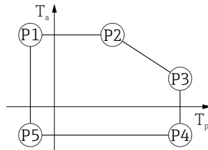
▣ 31 塑料外壳; 过程温度范围: -20 ... +200 °C (-4 ... +392 °F)
