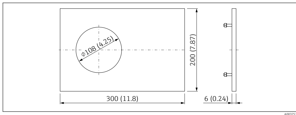
24 Baffle plate, 1.4301, sensor cut-out \varnothing 108 mm (4.25 in). Unit of measurement mm (in)
