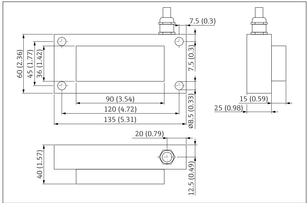
8 Dimensions. Unit of measurement mm (in)
