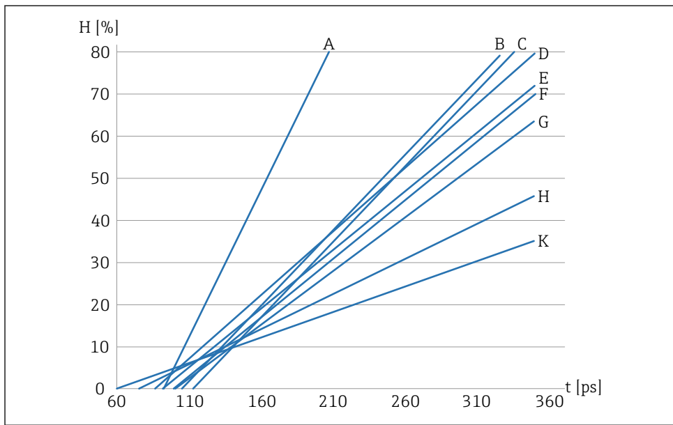
13 Kalibratiecurveset B (Cal.A, Cal.B, Cal.C, Cal.D, Cal.E, Cal.F, Cal.G, Cal.H, Cal.K)
