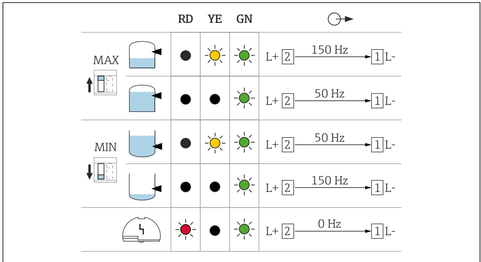
23 Switching behavior and signaling, electronic insert FEL67
