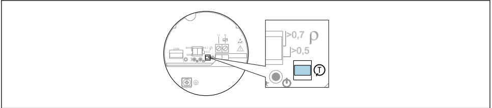
32 Position of key for the functional test for electronic inserts FEL61/62/64/64DC/67/68
