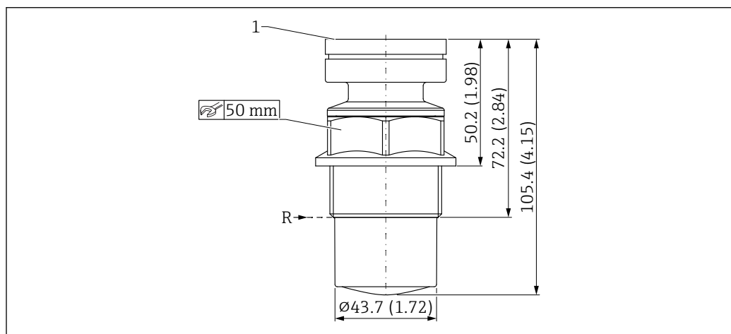
■ 24 Dimensions of encapsulated antenna, PVDF, 40 mm (1.5 in). Unit of measurement mm (in)
