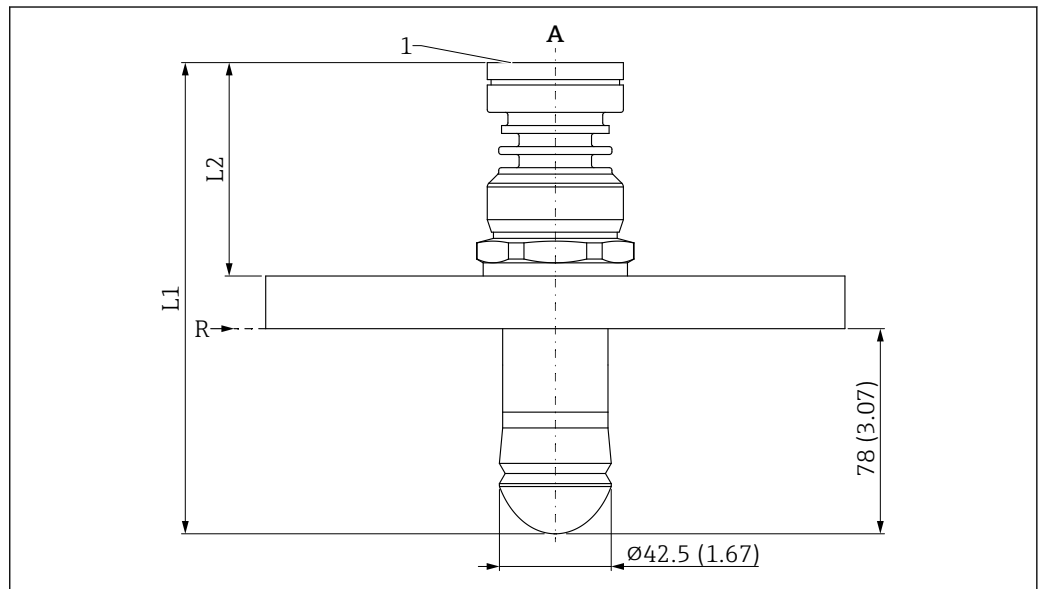
30 Dimensions of Drip-off antenna 50 mm (2 in), UNI flange process connection. Unit of measurement mm (in)
