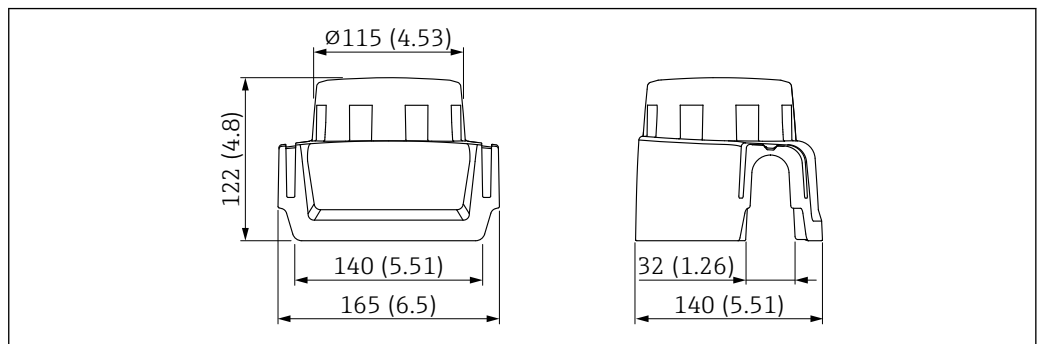
39 Dimensions. Unit of measurement mm (in)
