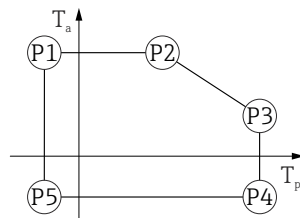
17 316L housing, hygiene; process temperature -40 to +80 °C ( -40 to +176 °F)
