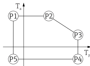
16 316L housing; process temperature -40 to +130 °C ( -40 to +266 °F)
