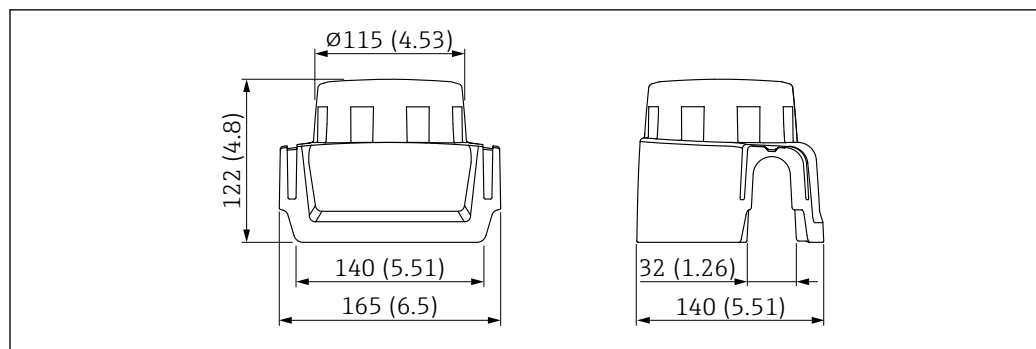
20 Protective cover for single compartment housing, aluminum or 316L. Unit of measurement mm (in)
