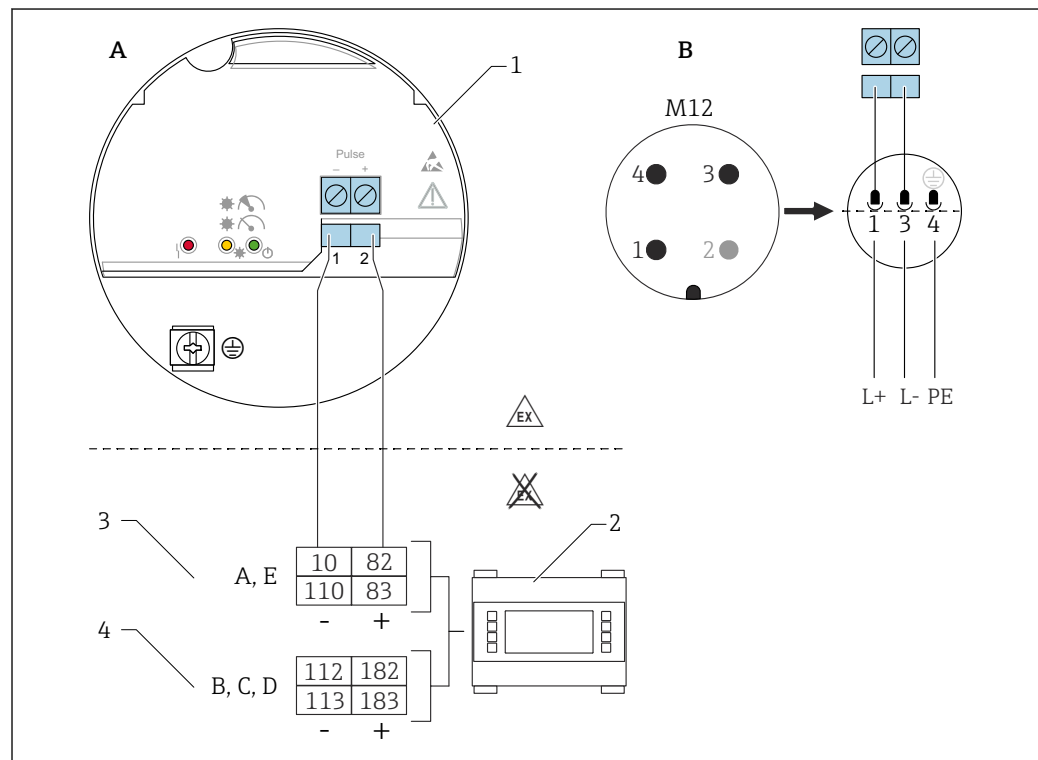
14 Connection diagram: electronic insert FEL60D connection to Density Computer FML621
