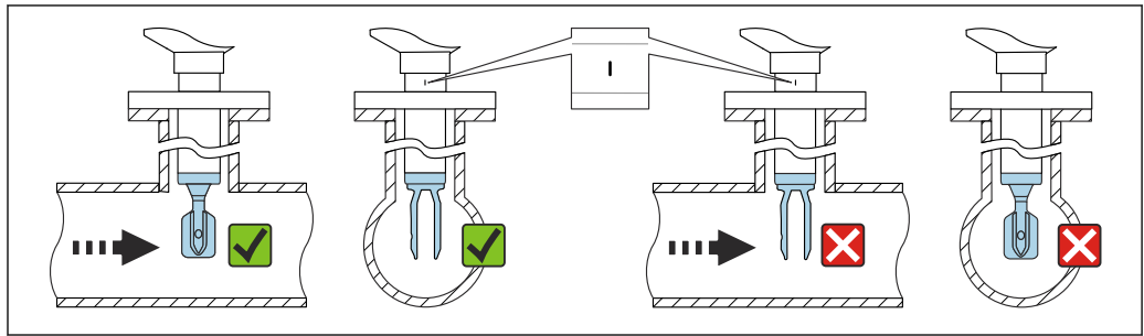
11 Installation in pipes (take fork position and marking into consideration)
