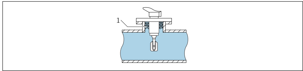
4 Installation example in pipes within the media flow
