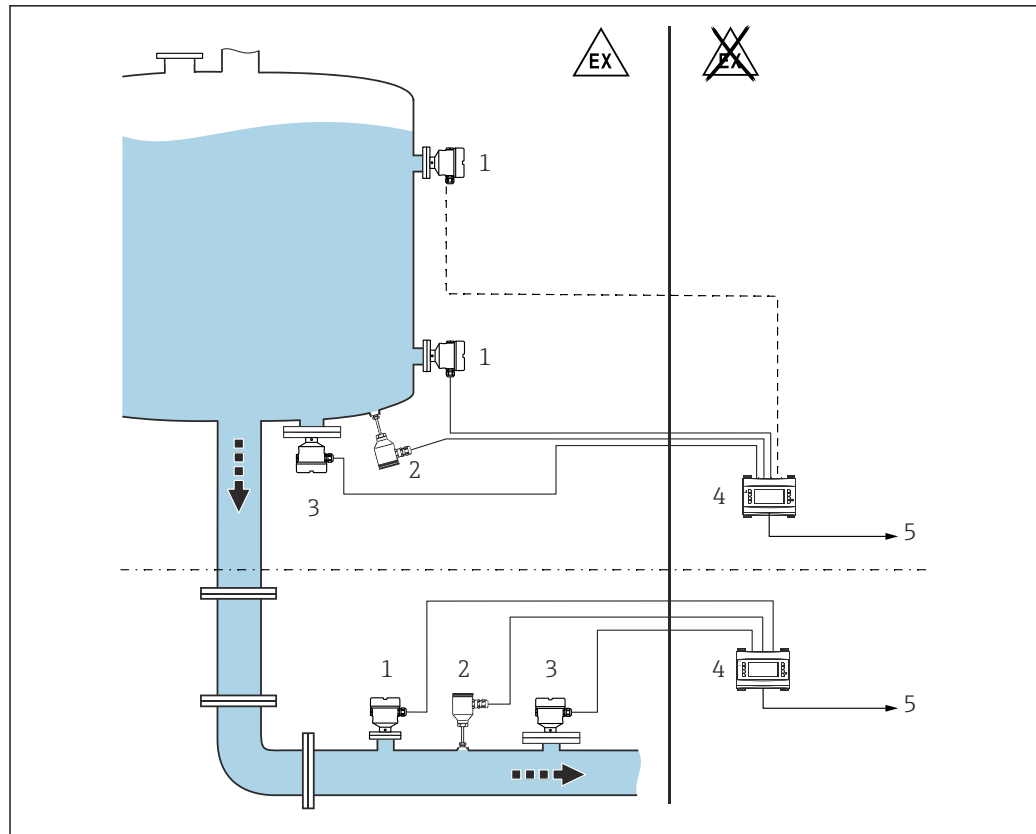
15 Density measurement with Density Computer FML621
