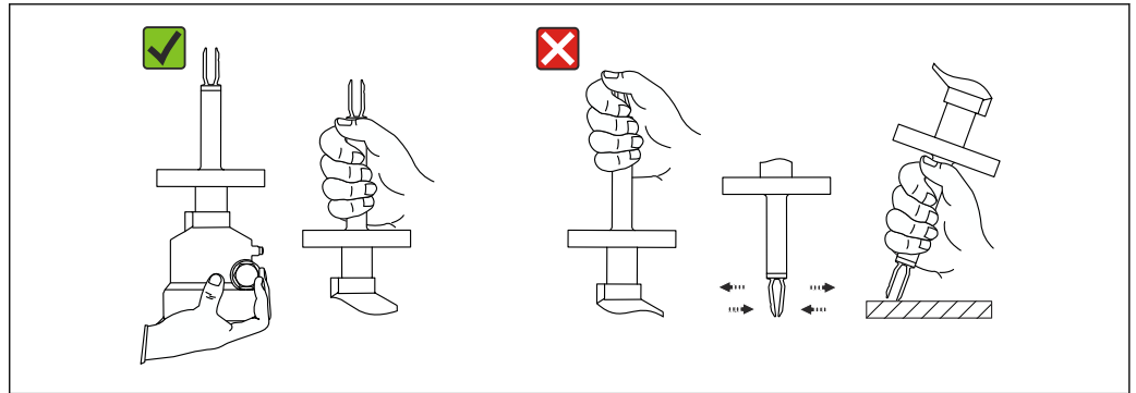
2 Handling the device during transportation
