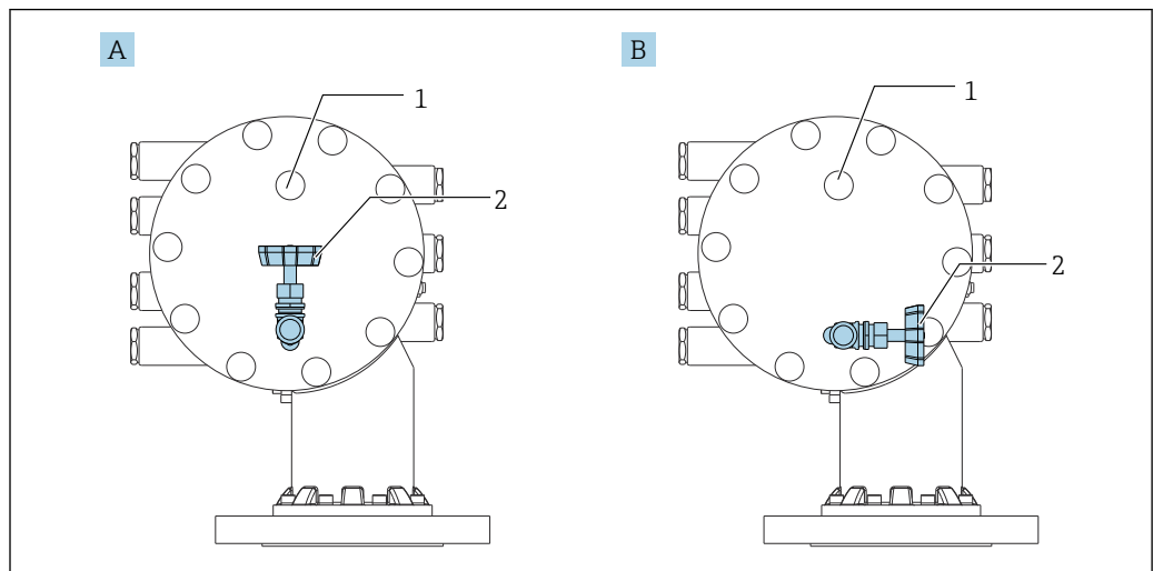
32 Cleaning nozzle and relief valve
