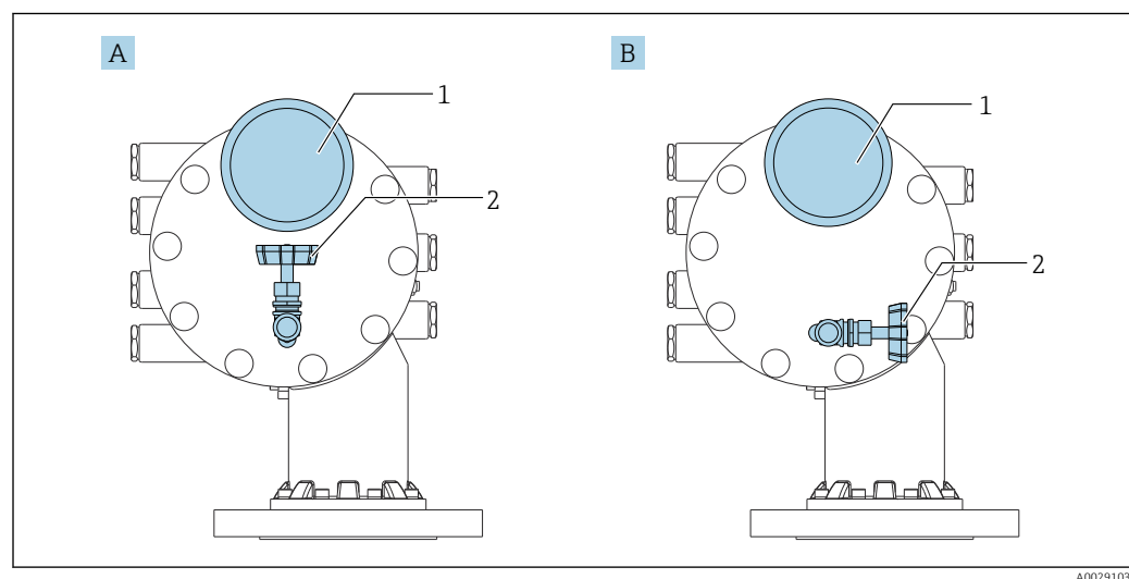
28 Mounting position of relief valve and pressure gauge
