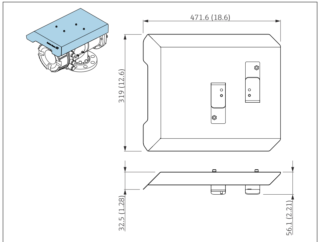
27 Weather protection cover; dimensions: mm (in)
