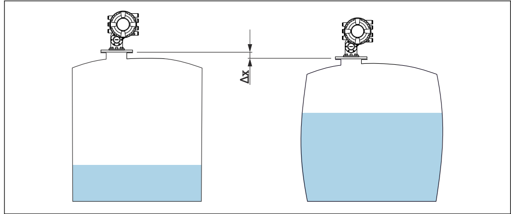
24 Movement \Delta x of the tank reference height due to the bulging of the tank shell caused by hydrostatic pressure
