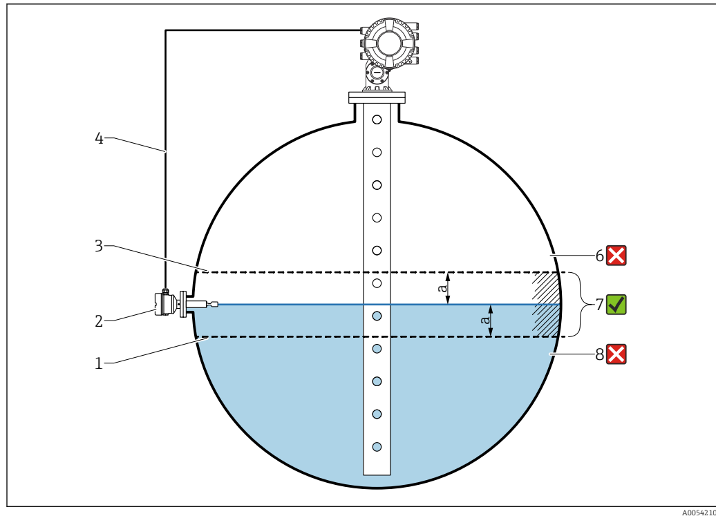
26 Application example with level switch
