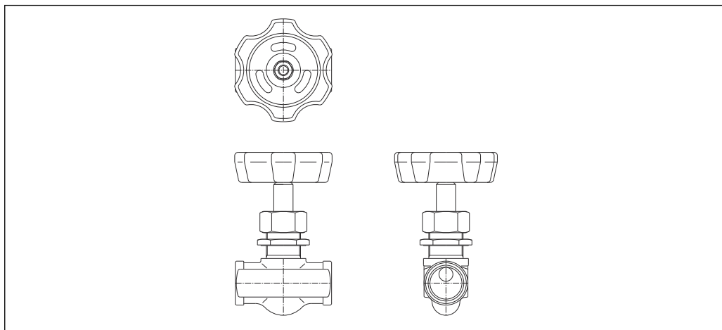
29 Relief valve
