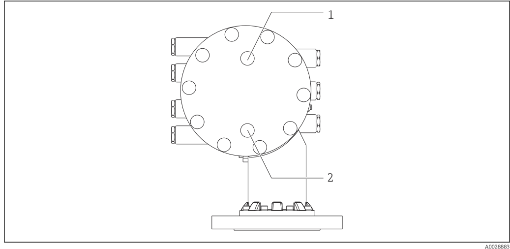
31 Holes for cleaning nozzle and gas purging nozzle
