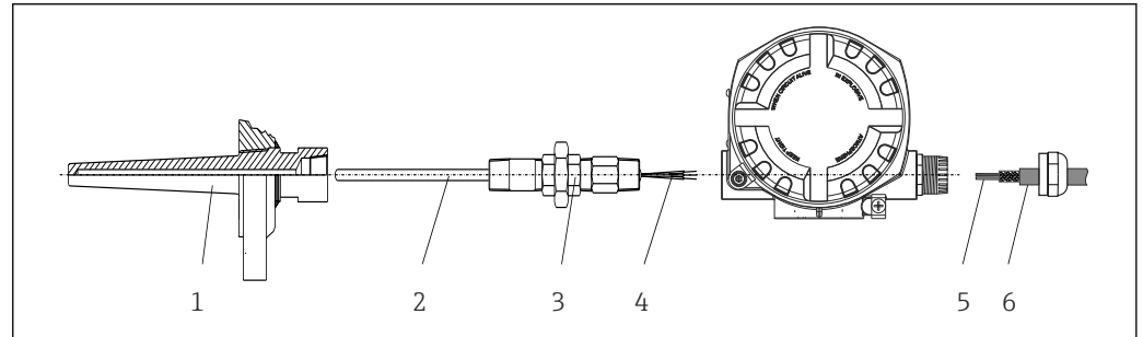
5 Direct field transmitter mounting on sensor
