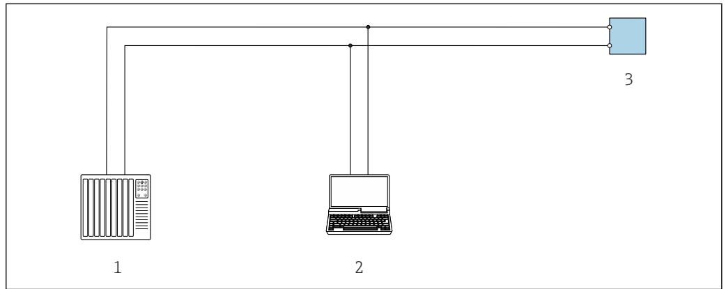
56 Options for remote operation via Modbus RS485 protocol (active)
