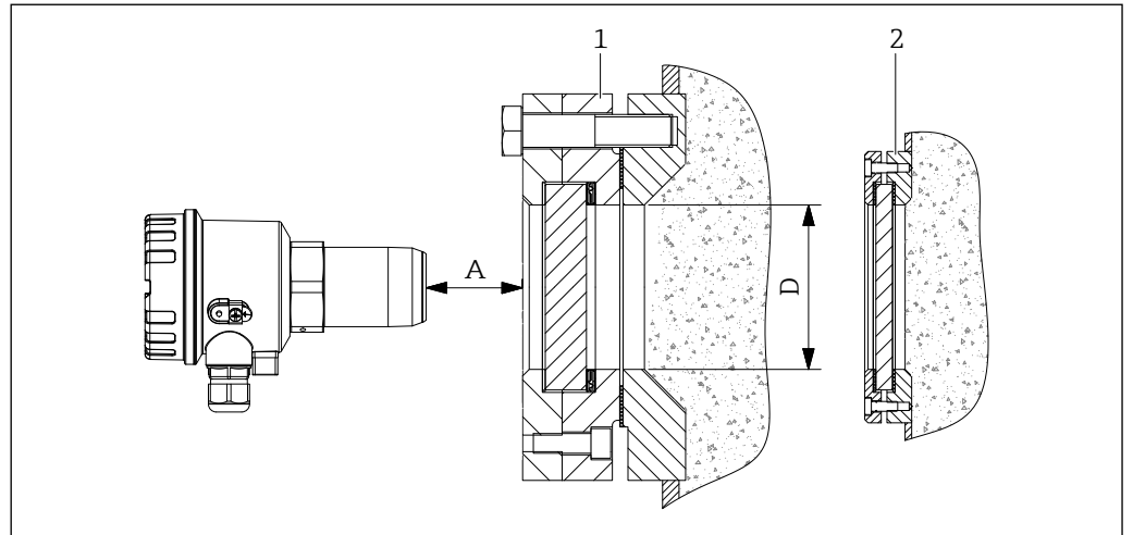
12 Mounting in front of microwave-permeable sight glass fitting
