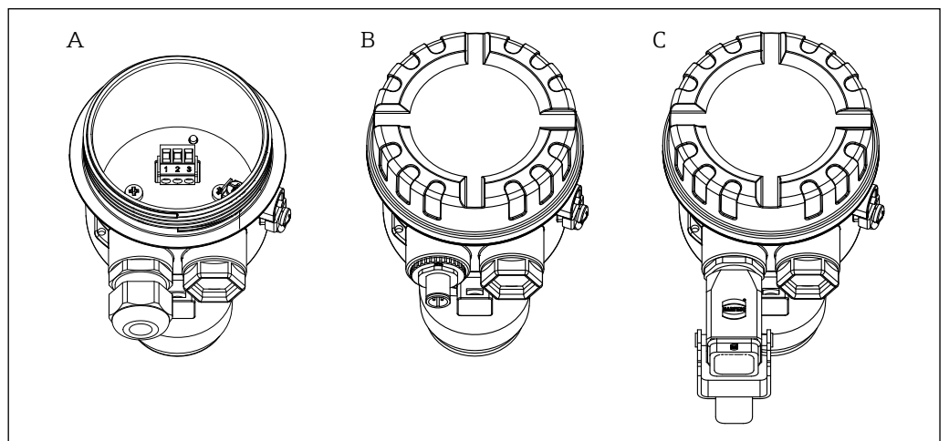
4 Terminal assignment
