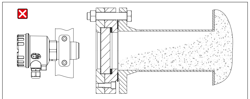
13 Impermissible mounting with the risk of material collection
