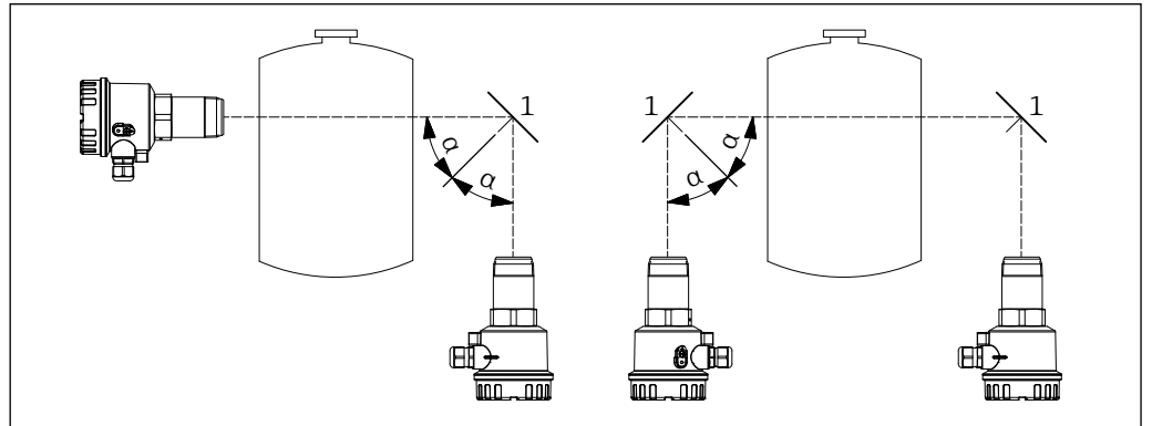
7 Reflector operation
