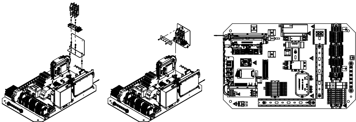
Figure 46. Electronics panel assembly parts (continued)
