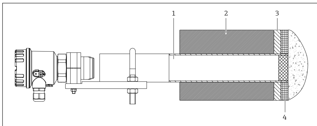
22. Mounting with spacer tube (wave guide)
