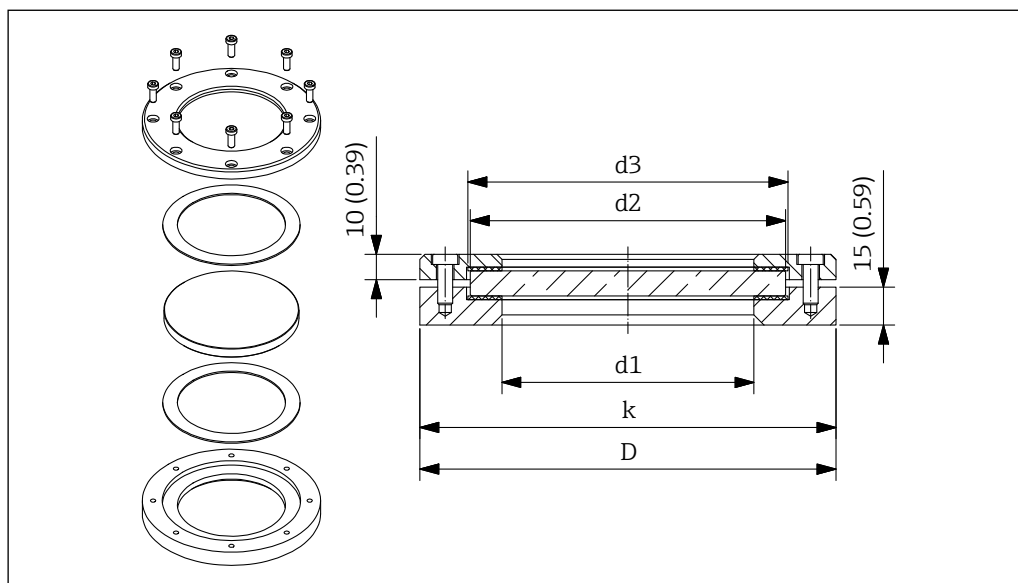
43 Dimensions sight glass fitting for unpressurized processes. Unit of measurement mm (in)
