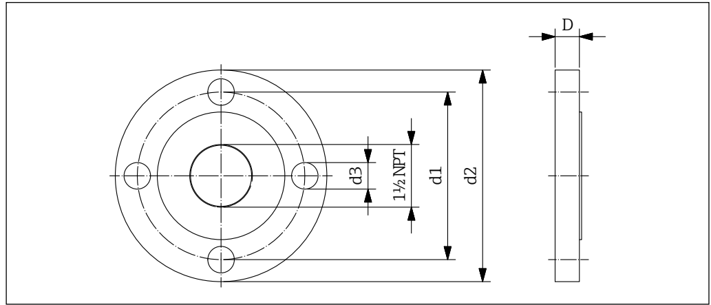
40 Dimensions mounting flange (Connection dimensions according to ANSI/ASME B16.5)
