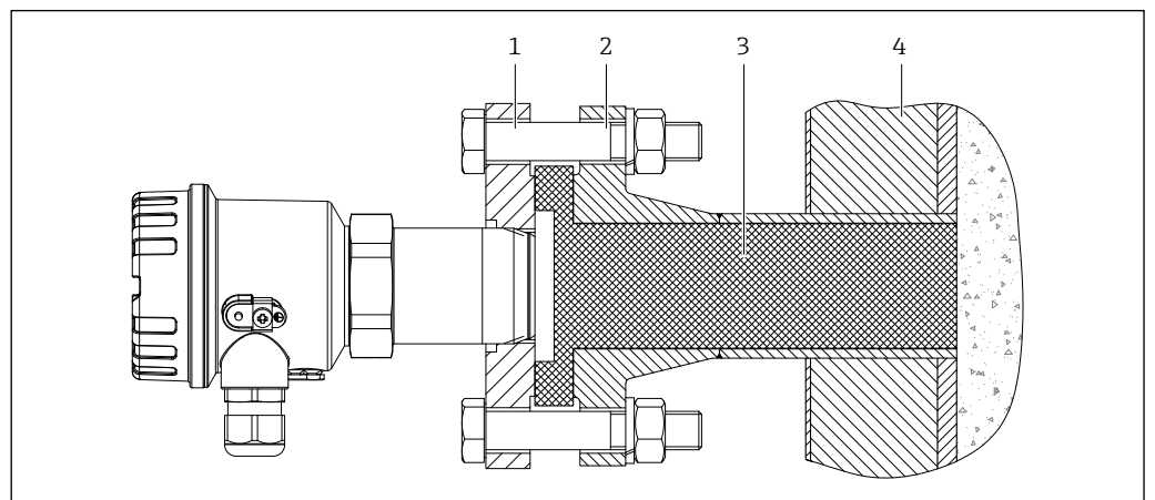
18 Weld-in nozzle FAR50
