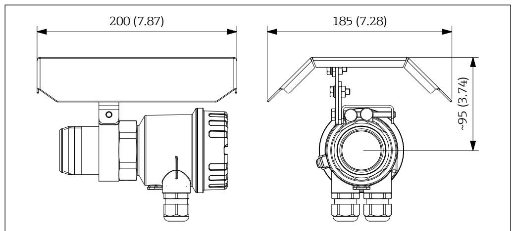
50 Dimensions weather protective cover. Unit of measurement mm (in)
