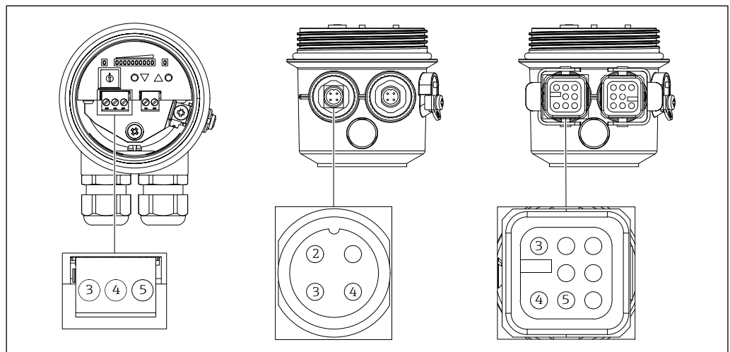
26 Connection signal circuit (Connector 2)
