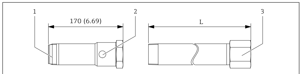
49 Dimensions high temperature adapter with extension. Unit of measurement mm (in)
