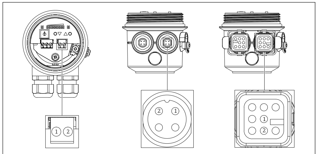
25 Supply circuit connection (Connector 1)
