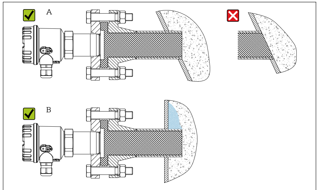
17 Mounting on process nozzle
