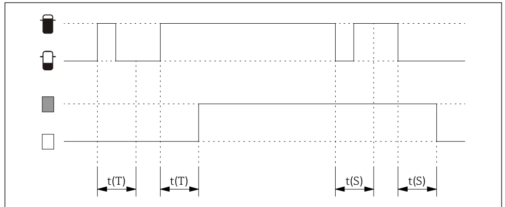
31 Adjustment of switching delays
