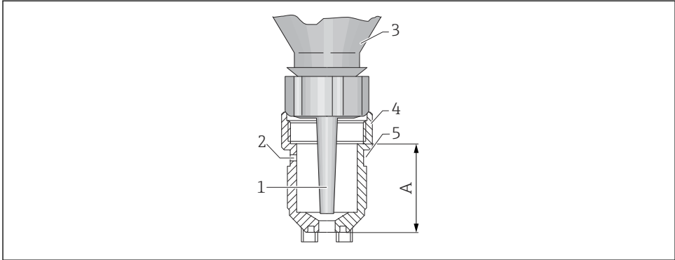
8 Membrane cap with electrolyte bottle
