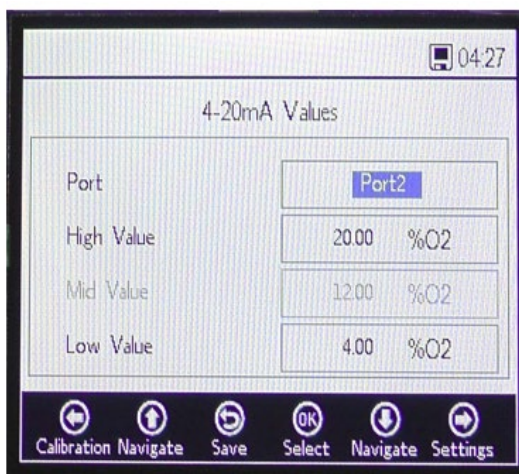
Figure 67. 4-20mA values for mode "Linear"
