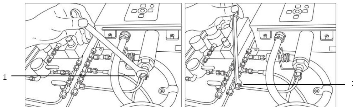
Figure 80. Removing the Swagelok nuts
