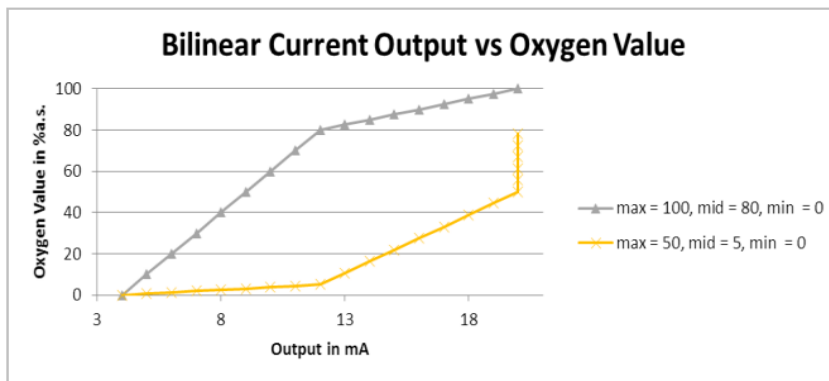
Figure 65. Bilinear current output vs oxygen value
