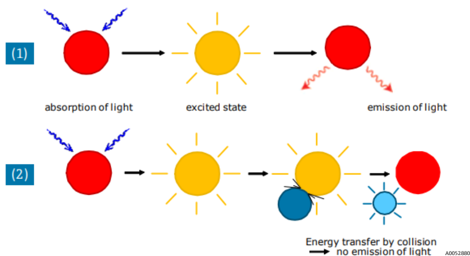
Figure 6. Principle of dynamic quenching of luminescence by molecular oxygen
