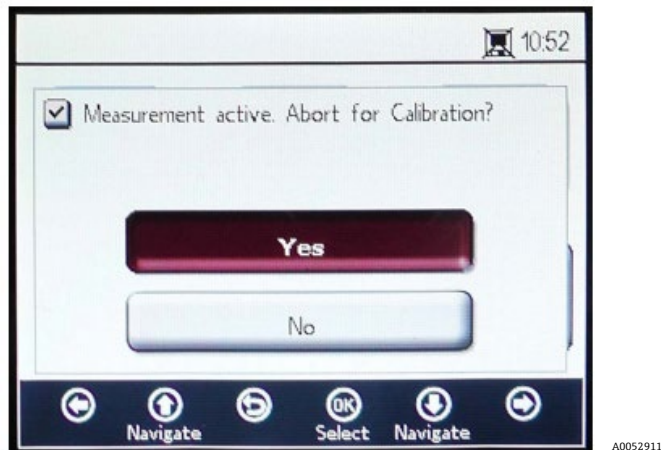
Figure 43. Message window - Stop measurements during configurations
