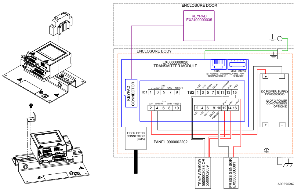
Figure 74. Interconnect diagram (DC)
