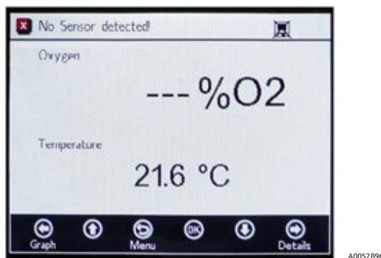
Figure 28. Error message - Sensor cannot be detected
