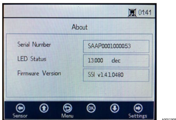
Figure 41. About screen
