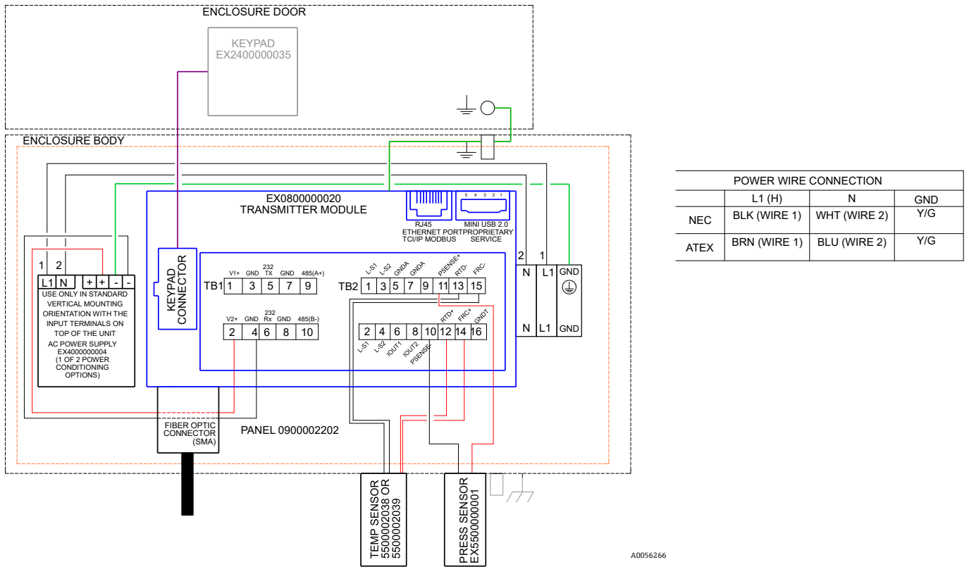
Figure 73. Interconnect diagram (AC)
