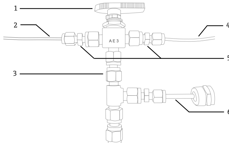
Figure 50. Gas inlet connections without SCS
