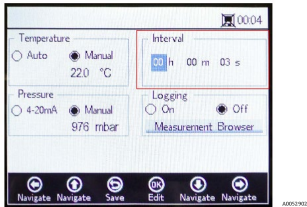
Figure 34. Measurement settings screen - Select time interval
