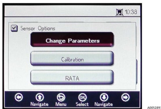
Figure 21. Sensor options
