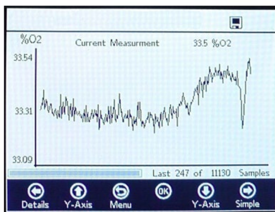
Figure 30. Graph screen
