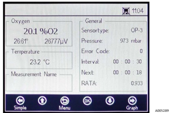
Figure 29. Details measurement screen
