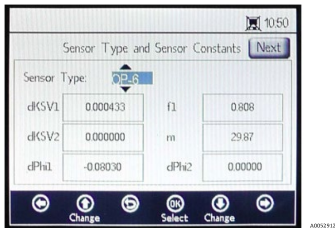
Figure 44. Sensor type and sensor constants - Sensor type menu selected for editing
