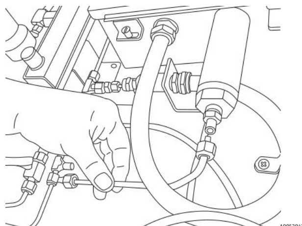
Figure 81. Removing the tubing
