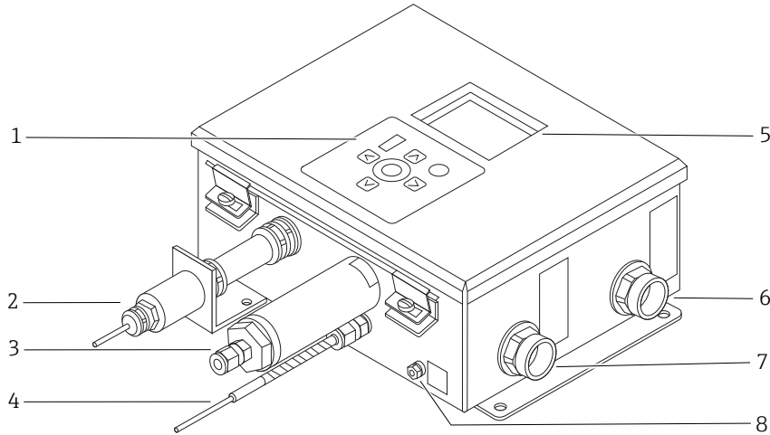
Figure 1. OXY5500 analyzer
