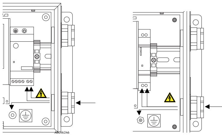
Figure 8. AC/DC power connections
