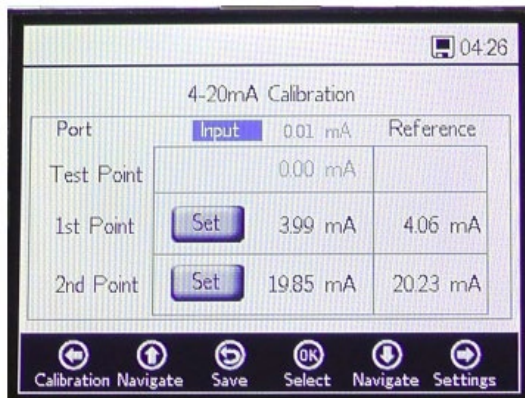
Figure 71. Analogues - 4-20mA input calibration
