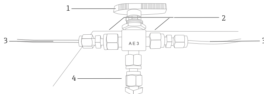
Figure 51. Gas inlet connections with SCS
