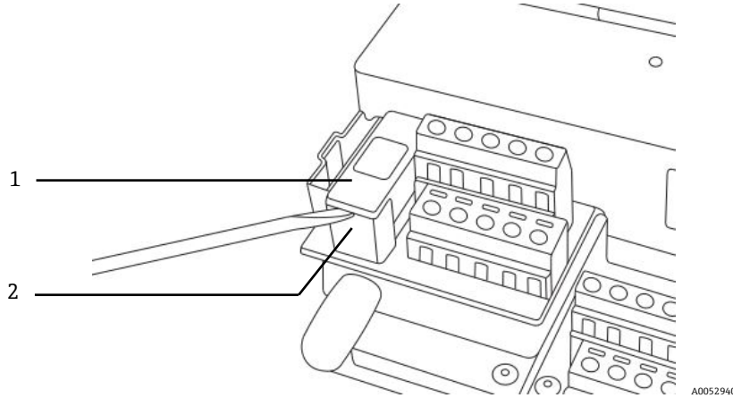
Figure 75. Removing the fuse cover
