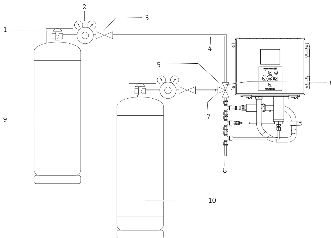
Figure 49. General layout for cylinder and Endress+Hauser analyzer connections
