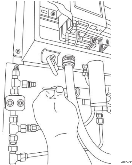
Figure 88. Remove probe from tee union (panel side)
