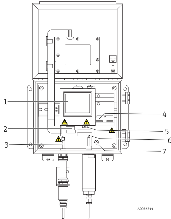
Figure 3. Inside cabinet view (AC version)
