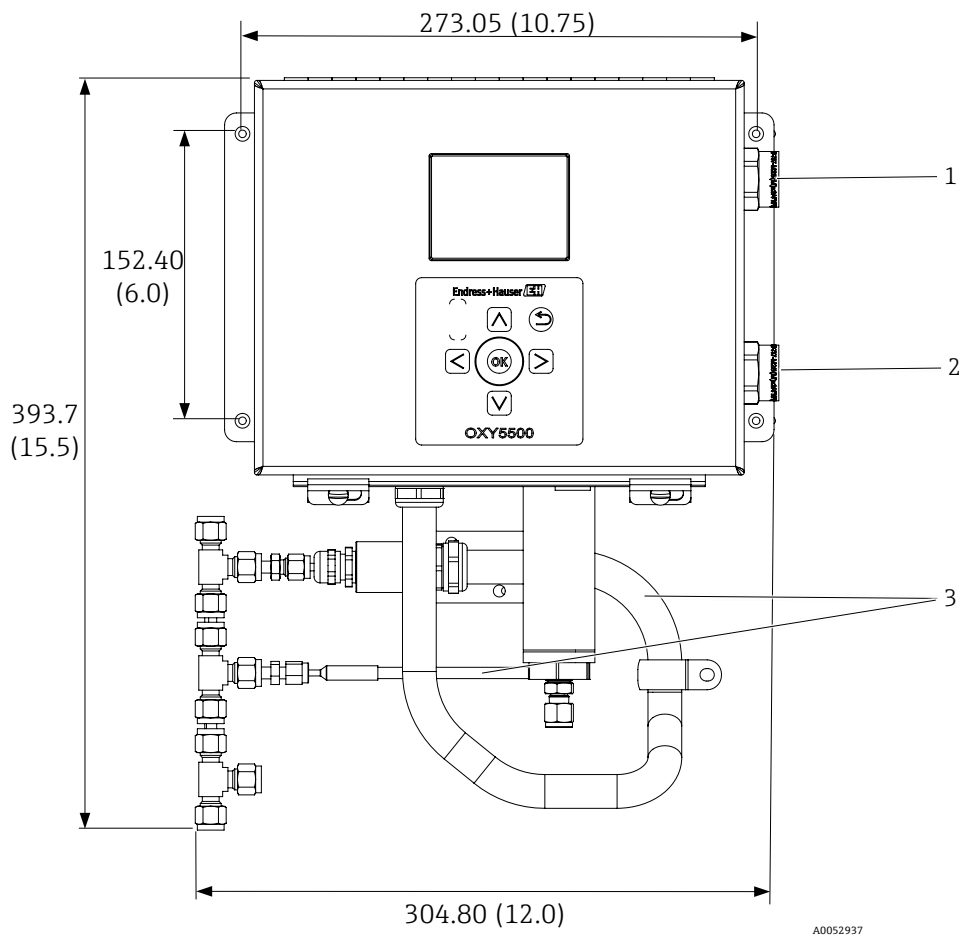
Figure 72. Outline and mounting dimensions - panel mount. Dimensions: mm(in)
