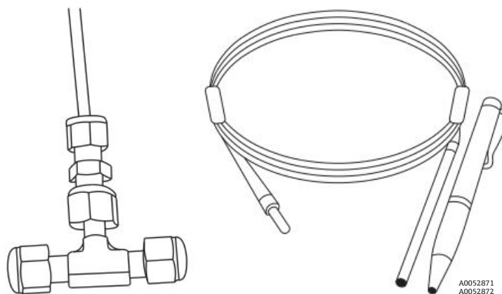
Figure 5. Standard fiber-optic oxygen sensors fittings
