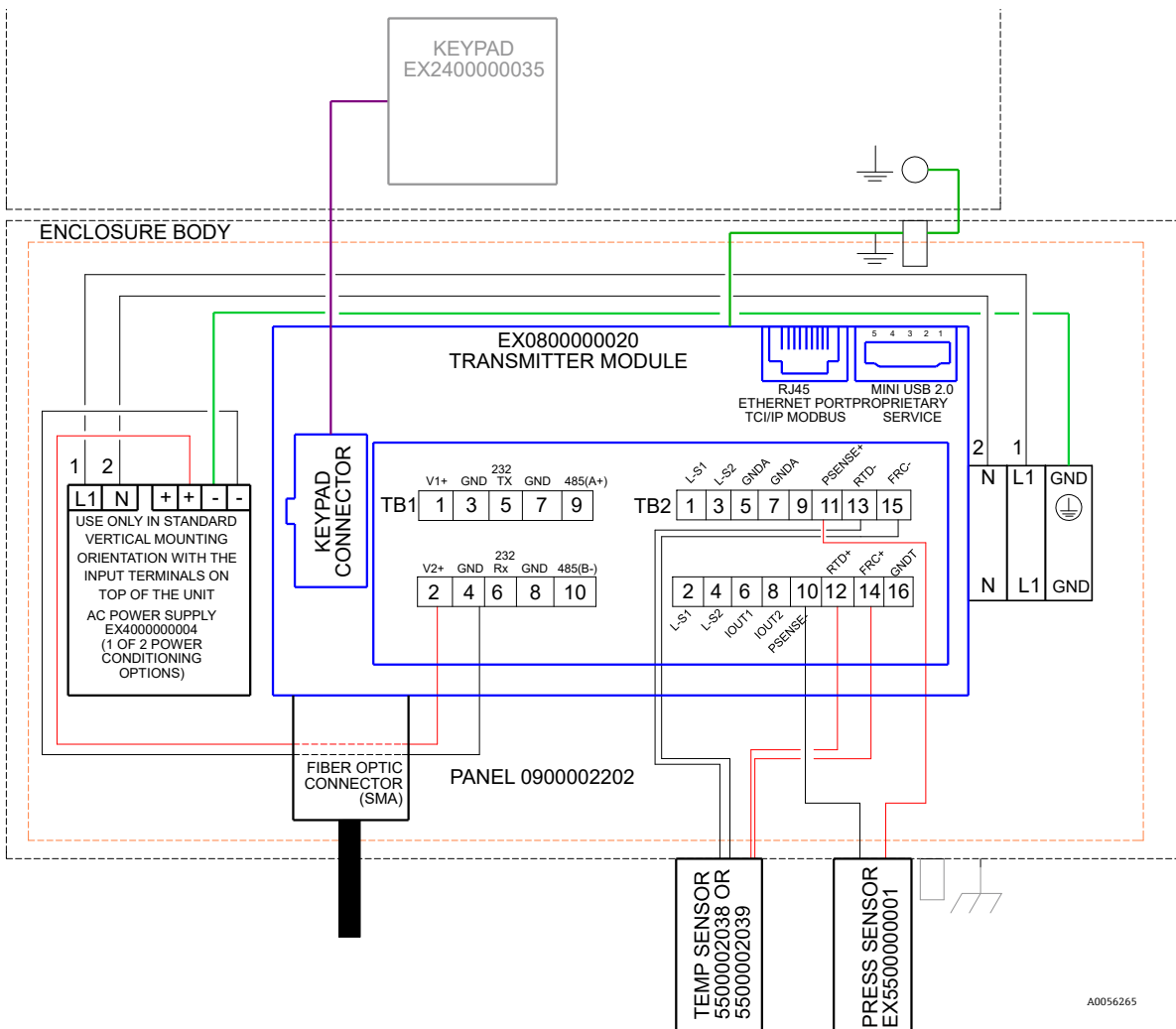
Figure 10. TB1/TB2 connections
