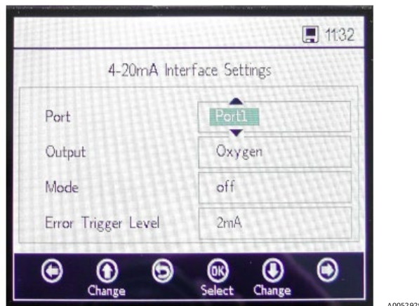
Figure 64. Analogues - 4-20mA interface settings
