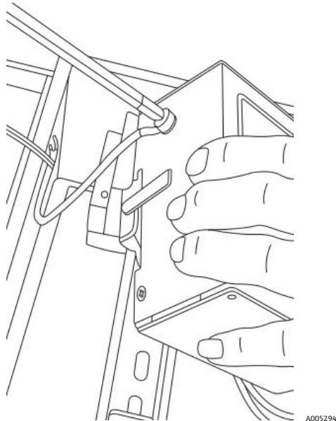
Figure 79. Removing the ground cable
