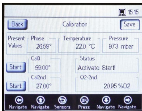
Figure 56. Calibration screen
