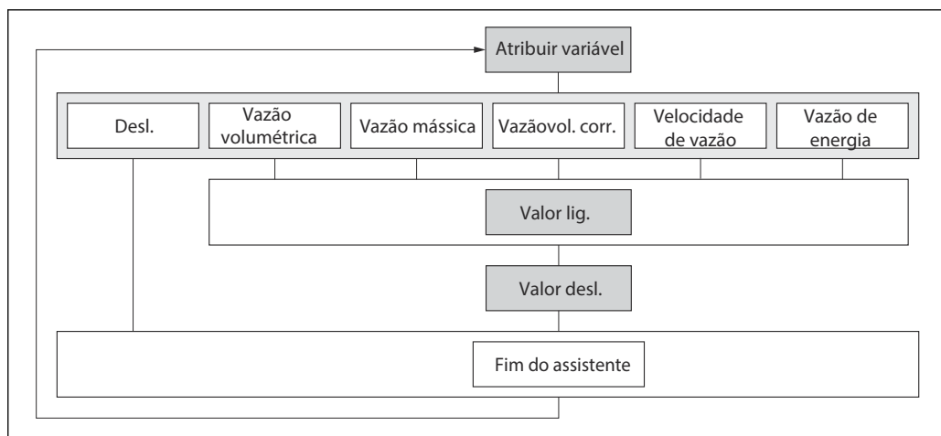
31 Assistente "Low flow cutoff" no menu "Setup"
