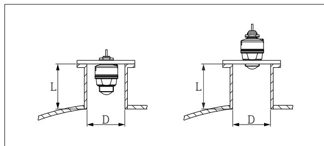
2 Nozzle installation, 40 mm (1,5 in) antenna
