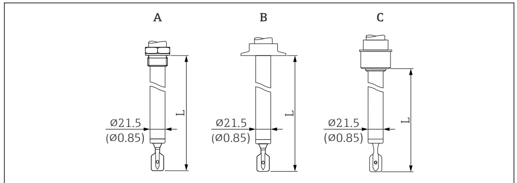
i 17 Probe designs: pipe extension, short pipe (sensor length L). Unit of measurement mm (in)
