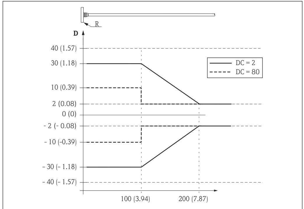
21 Measurement error at the upper probe end; unit: mm (in)
