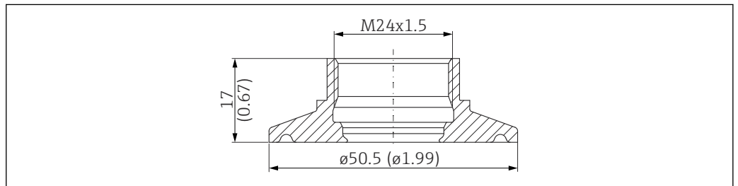
34 Tri-Clamp ISO2852 DN25-38 (1 to 1½"), 316L. Unit of measurement mm (in)
