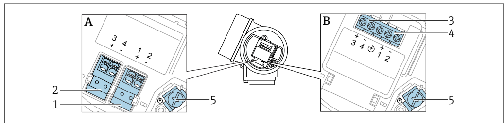
6 Terminal assignment, 2-wire: 4 to 20 mA HART, switch output
