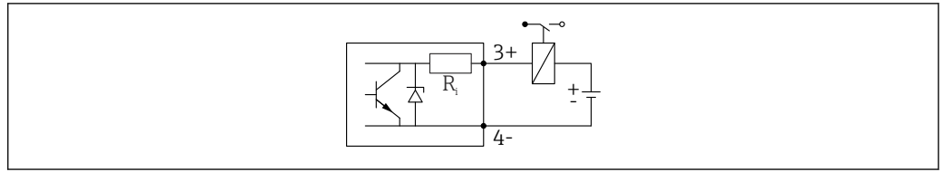
8 Connection example of relay
