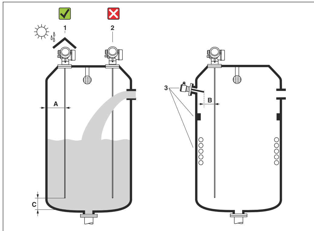
22 Installation positions
