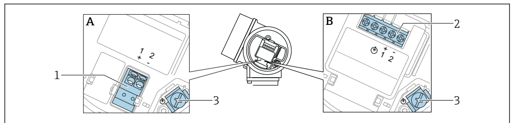
4 Terminal assignment, 2-wire: 4 to 20 mA HART
