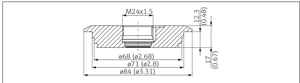
37 Varivent N pipe DN40-162 PN16, 316L. Unit of measurement mm (in)
