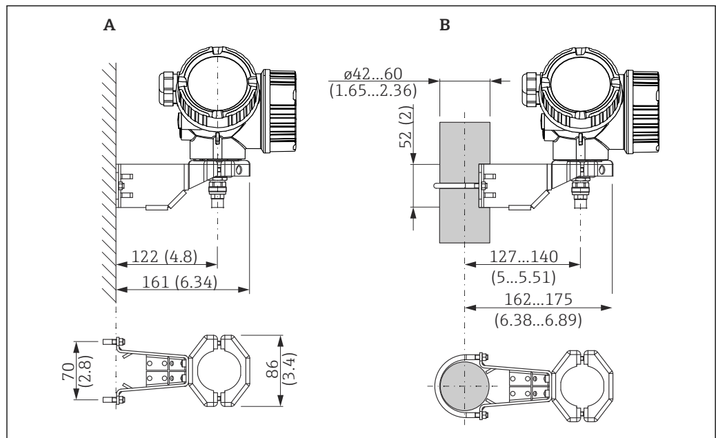
57 Mounting bracket for electronics housing; unit: mm (in)
