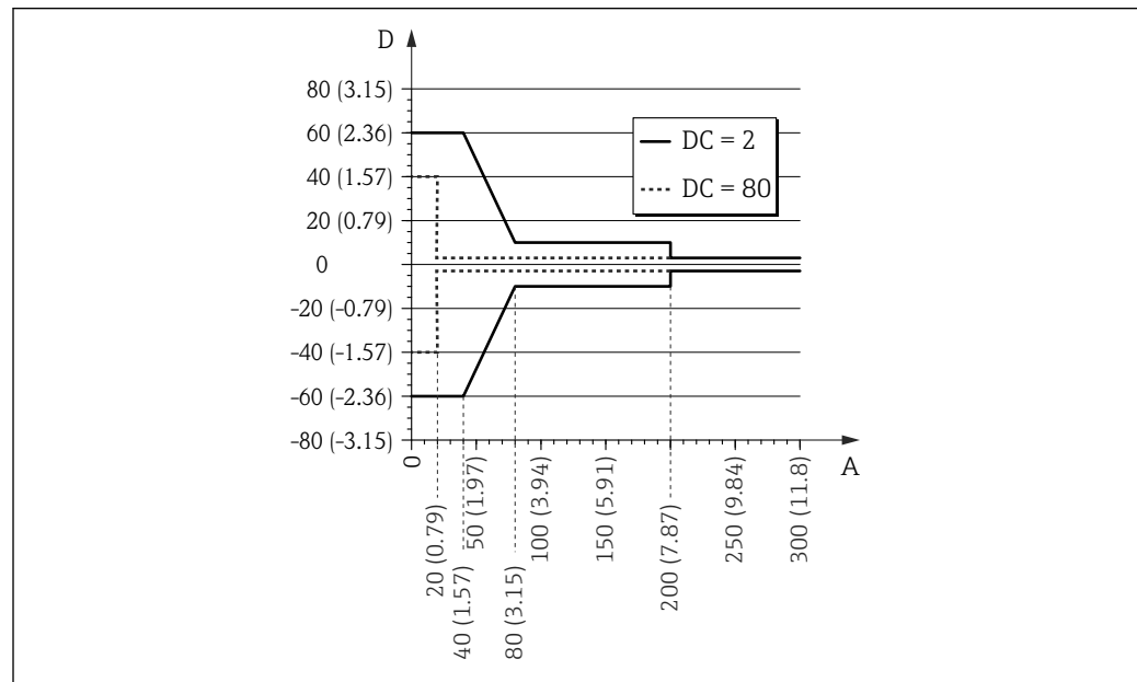
20 Measurement error at the probe end for rod and coaxial probes
