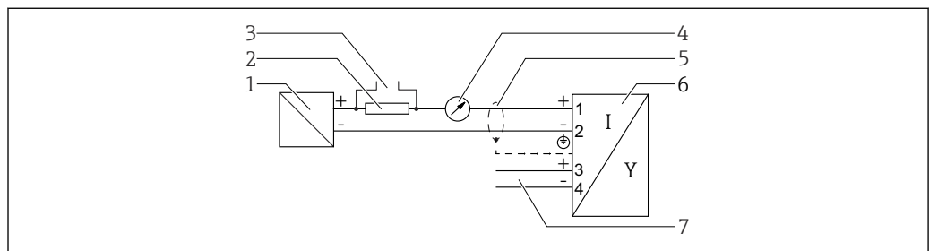
7 Function diagram 4 to 20 mA HART, switch output
