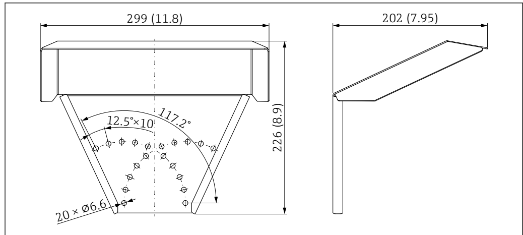
56 Dimensions. Unit of measurement mm (in)
