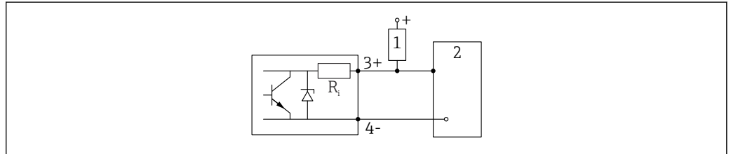
9 Connection example for the digital input
