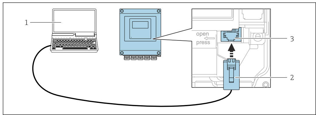
46 Raccordement via interface service (CDI-RJ45)
