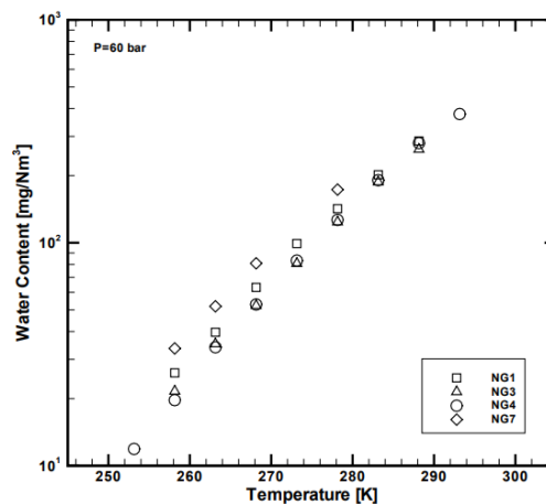
Courses of measured water contents at 60 bar for natural gas mixtures NG1, NG3, NG4, and NG7.
