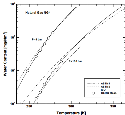
Comparison of calculation results for ASTM1 [8], ASTM2 [9] and ISO [10] methods with experimental data from the GERG report [14] for mixture NG4.
