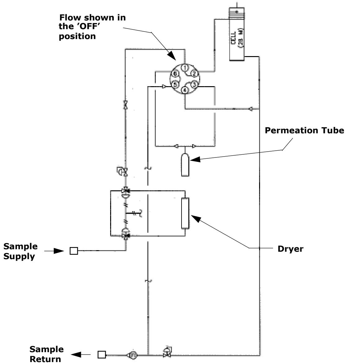
Figure 17. Typical sample system for differential measurement with permeation tube validation capability.
