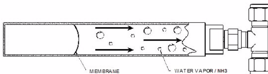
Figure 16. Permeation tube
