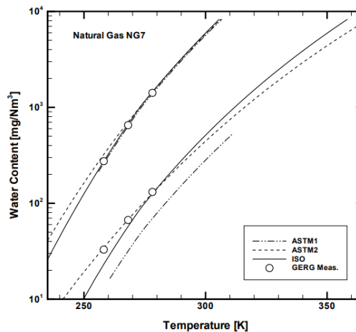
Comparison of calculation results for ASTM1 [8], ASTM2 [9] and ISO [10] methods with experimental data from the GERG report [14] for mixture NG7.
