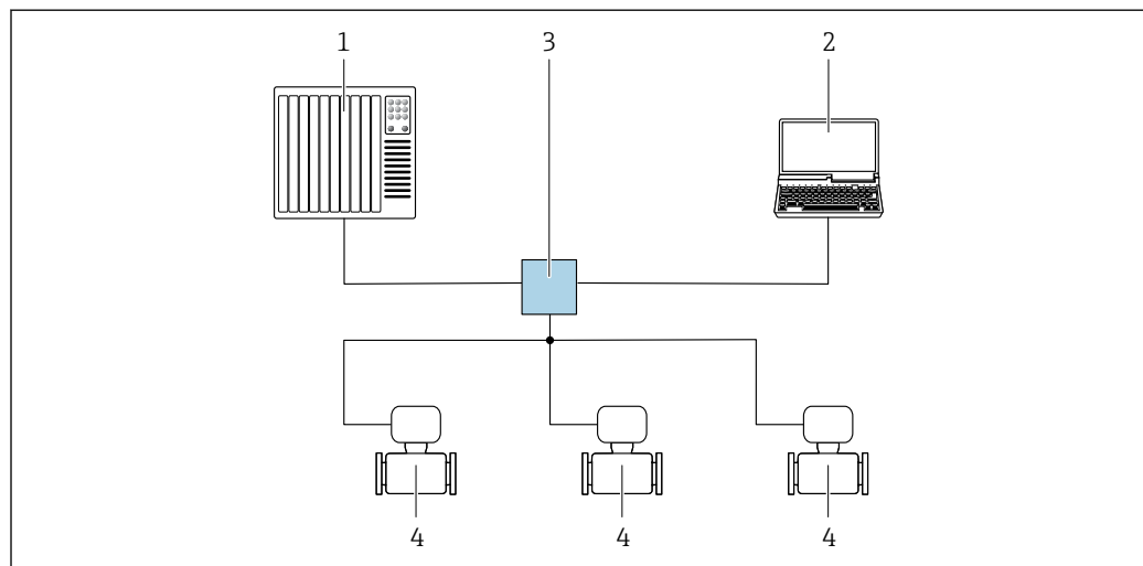
39 Options for remote operation via PROFINET network: star topology
