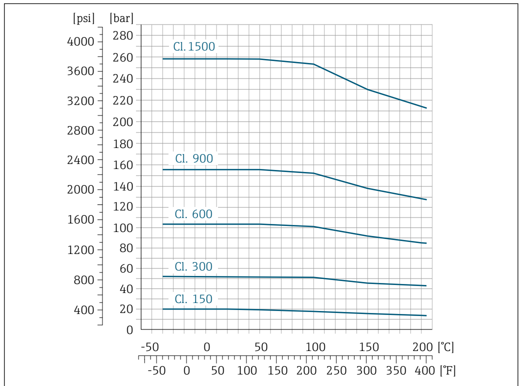
32 With flange material stainless steel, 1.4410/F53 25Cr Duplex (Super Duplex)
