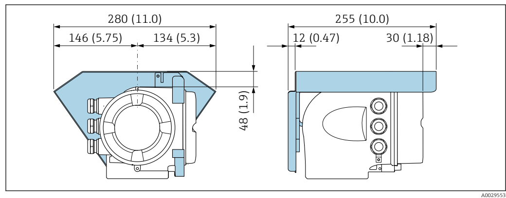
30 Weather protection cover for Proline 500; engineering unit mm (in)
