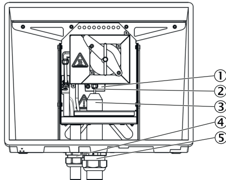
Figure 8: Sample gas connection SFU-BF NI GL in weatherproof enclosure
