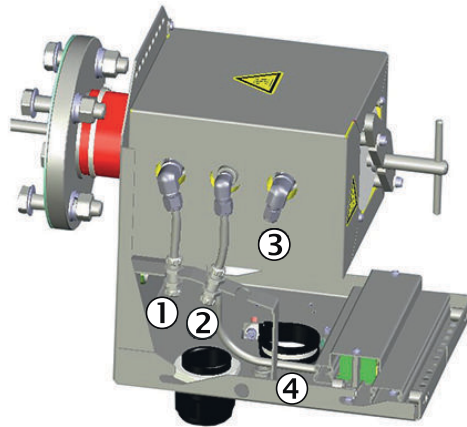
Figure 9: Connection of SFU-BF NI GL pneumatic lines
