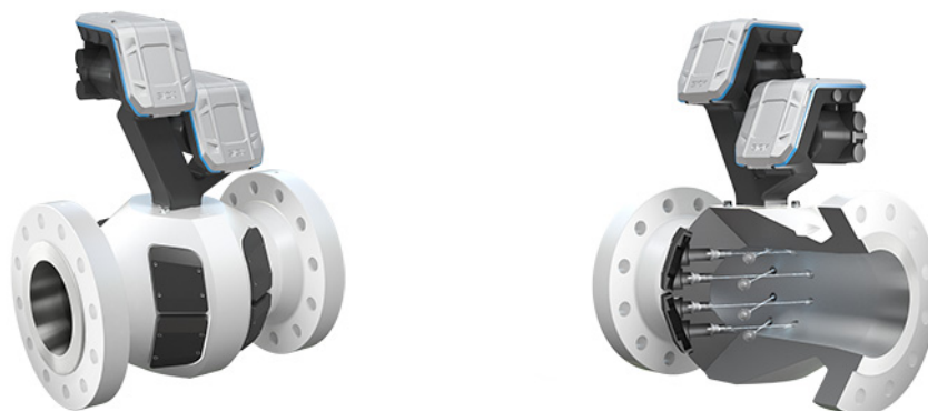
图 7 FLOWSIC600-XT Quatro
