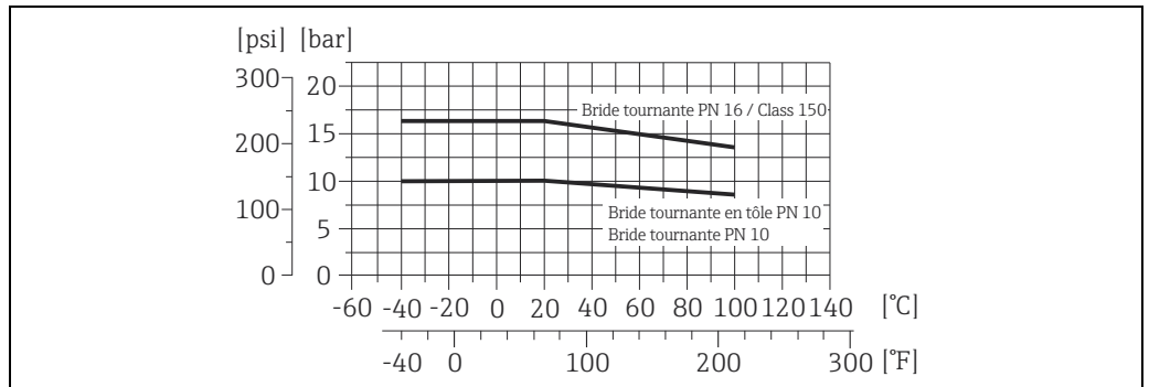
Matériau raccord process : acier inox (min. -40 °C (-40 °F)), acier au carbone (min. -10 °C (+14 °F))
