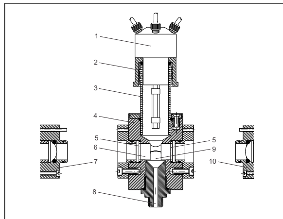
16 Side view of optics chamber
