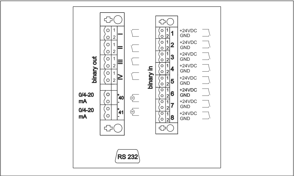
6 Signal connection
