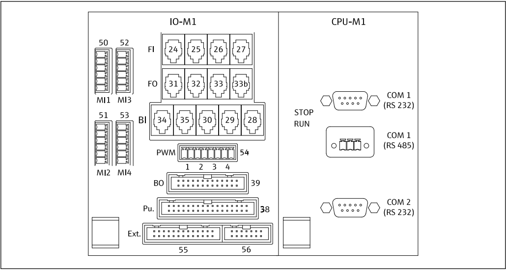
8 Distributor (* = pin 1 for MI1 - MI4 and for PWM)
