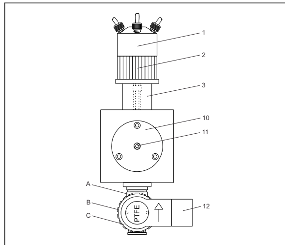
17 Front view of the measuring chamber
