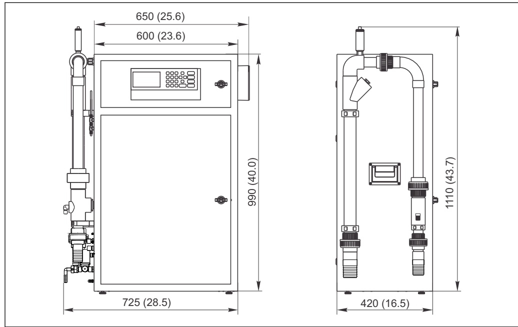
1 CA72TP analyzer with sample conditioning, dimensions in mm (inch)
