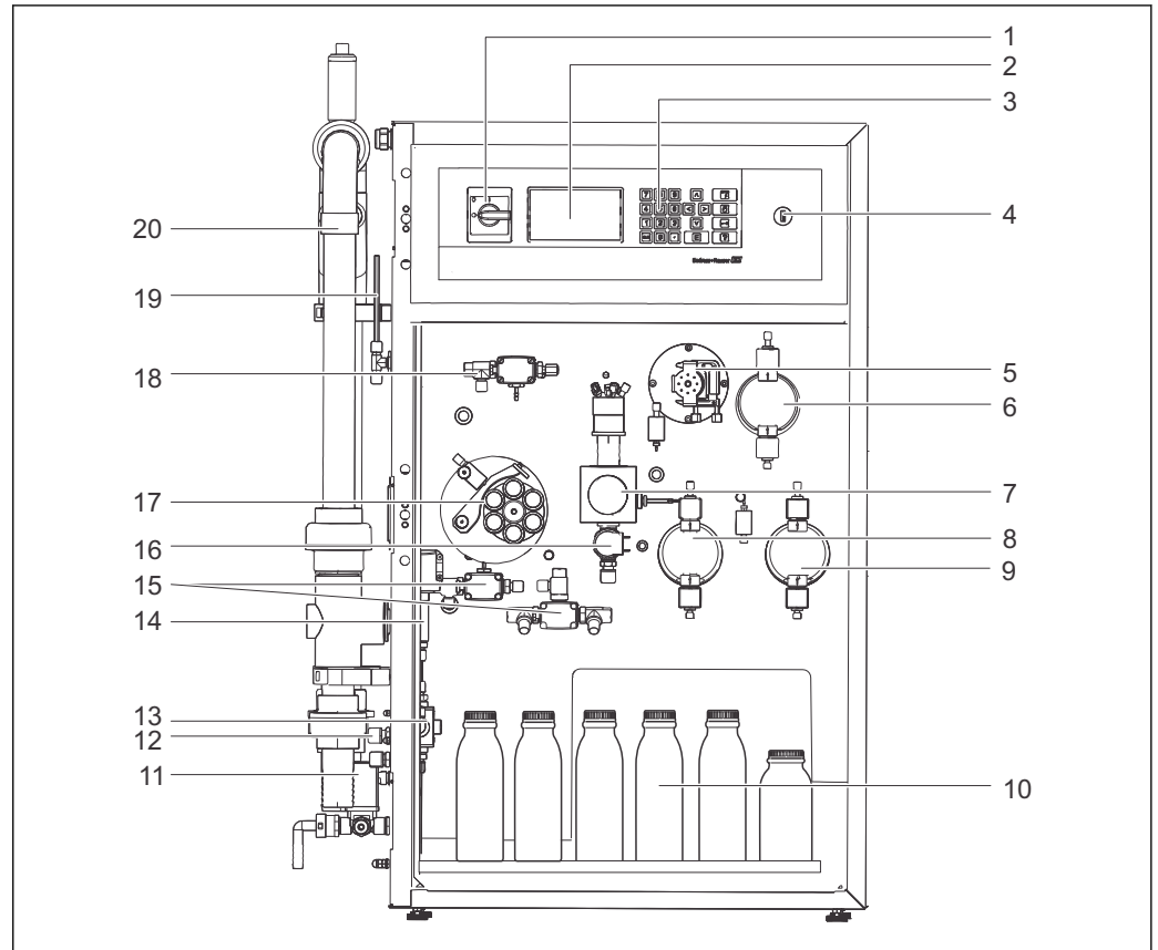
9 Analyzer, front view
