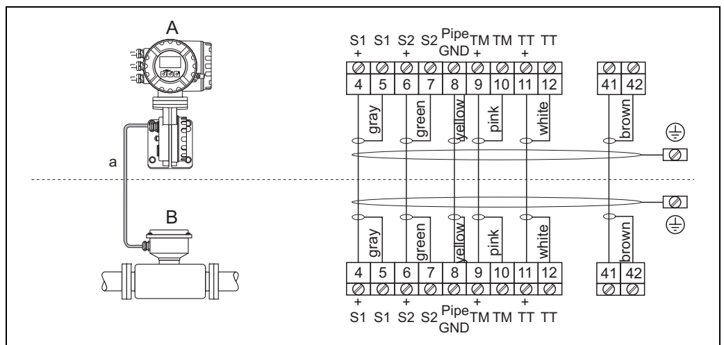
Fig. 3: Connection of connecting cable (remote version) A Transmitter remote version B Remote version connection housing a Sensor cable
