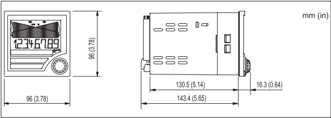
Fig. 24: Data in mm (data in inches in brackets)
