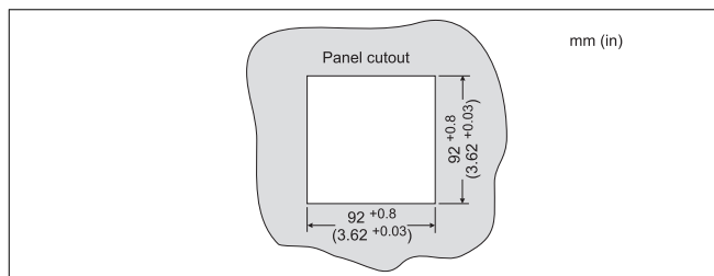
Fig. 3: Panel cutout (data in mm, data in inches in brackets)
