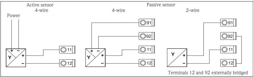
Fig. 8: Connecting a sensor to universal input
