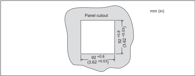
Fig. 25: Panel cutout (data in mm, data in inches in brackets)
