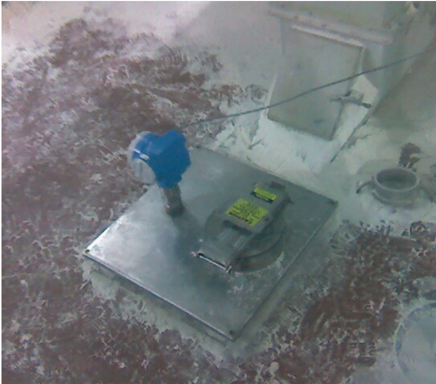
Levelflex M FMP40 installation at milling plant
