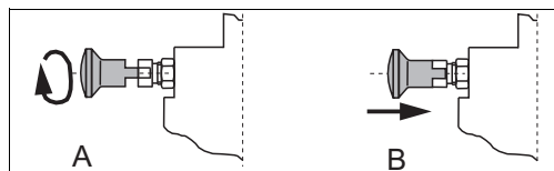
Fig. 14: Stop bolt
