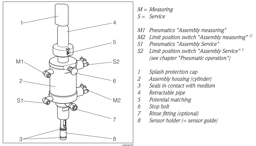
Fig. 9: Operating elements
