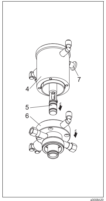
Fig. 21: Dismantling part 3
