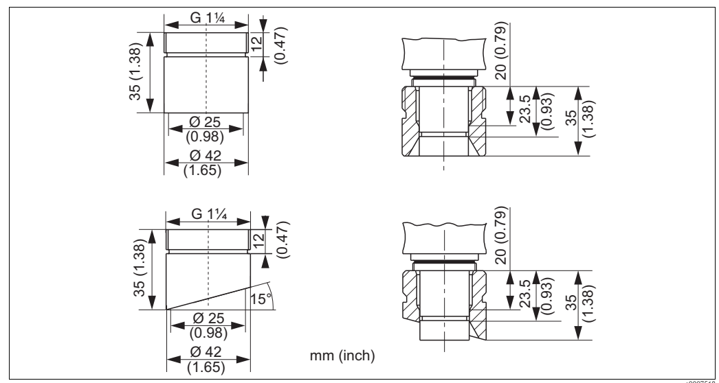
Abb. 23: Welded fittings
