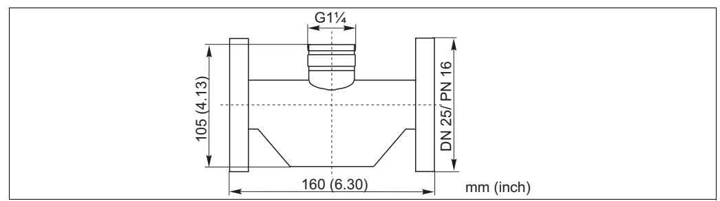
Fig. 24: Flow vessel
