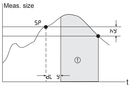
Operation of the time delay dL_{\text{Y}} / dL_{\text{N}}
