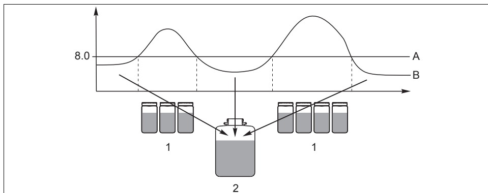
Fig. 8: Event-controlled sampling
