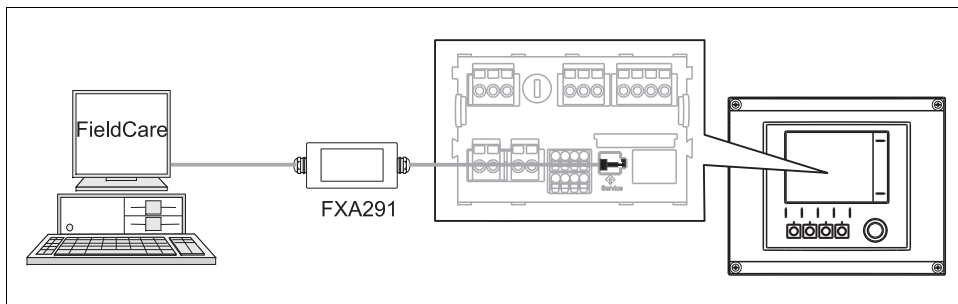
Fig. 11: Connection overview
