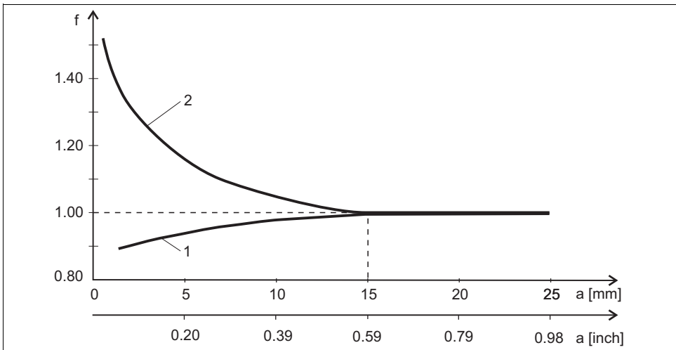
Fig. 14: Relation between the installation factor f and the wall distance
