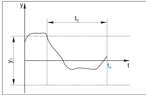
Fig. 13: Stagnating signal, alarm is triggered
