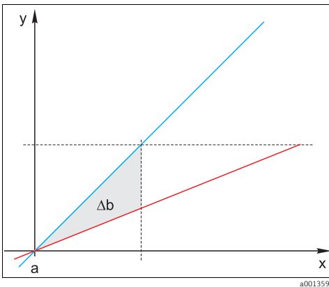
Fig. 5: Delta slope
