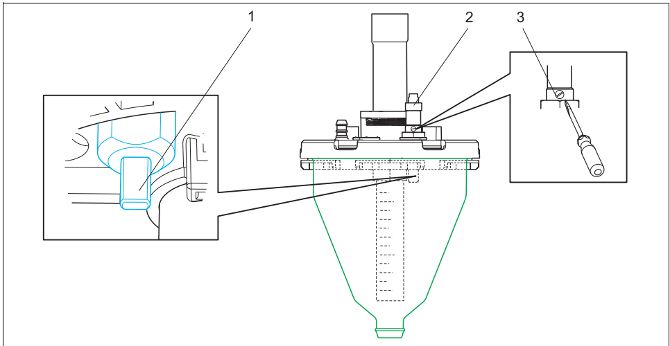
Fig. 3: Adjust the capacitance sample sensor
