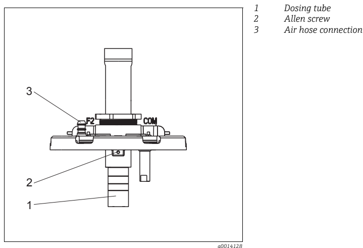
Fig. 2: Vacuum pump
