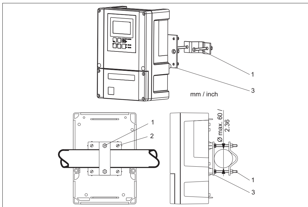
Fig. 5: Post mounting field device to cylindrical pipes
