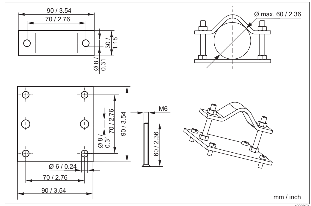
Fig. 37: Post mounting kit
