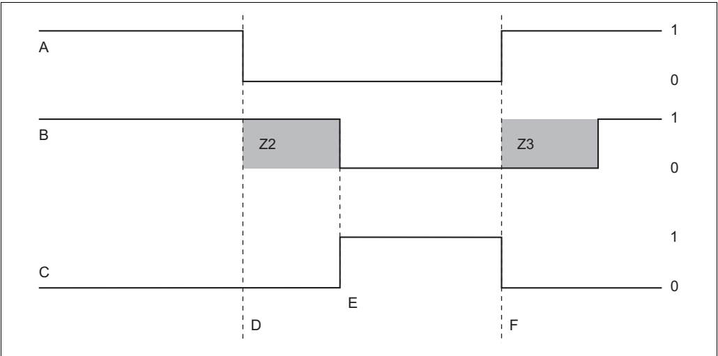
Fig. 20: Alarm signalling and dosing switch-off by the main stream A Flow in main stream F Flow restoration B Relay contacts of PID controller Z2 Delay for controller switch-off, see field Z2 C Alarm relay Z3 Delay for controller switch-on, see field Z3 D Flow below switch-off limit Z4 or flow failure 0 Off E Flow alarm 1 On
