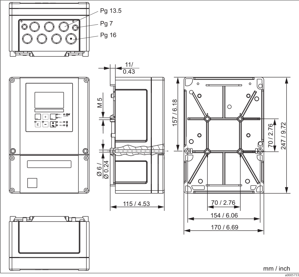
Fig. 1: Field instrument
