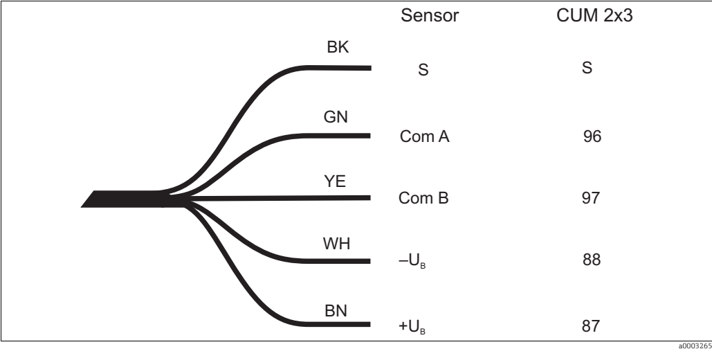
Fig. 11: Structure of measuring cable CYK8 and CYK81 (extension cable)
