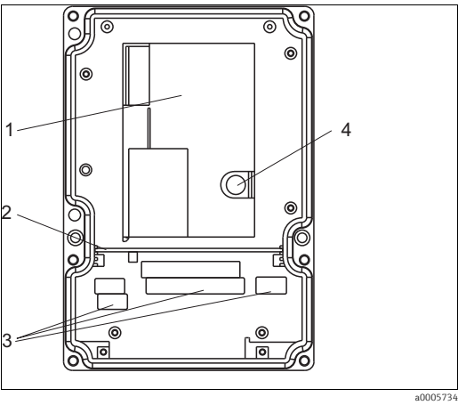
Fig. 2: View into the field housing
