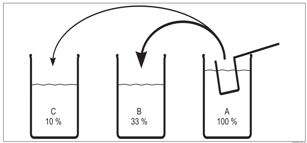
Fig. 31: Making the samples for a three-point calibration
