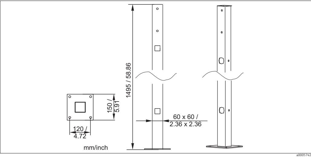
Fig. 36: Universal post
