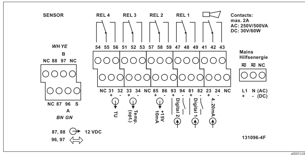
Fig. 9: Field instrument connection compartment sticker
