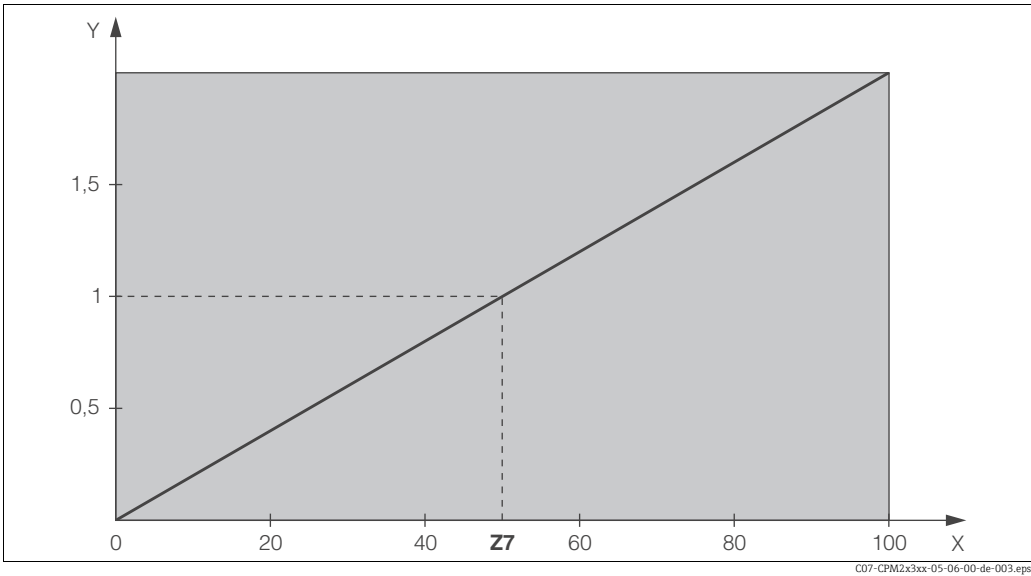
Fig. 22: Multiplying feedforward control Y Gain K_{inff} X Current input signal [%] Z7 Input value, when gain K_{inff} = 1
