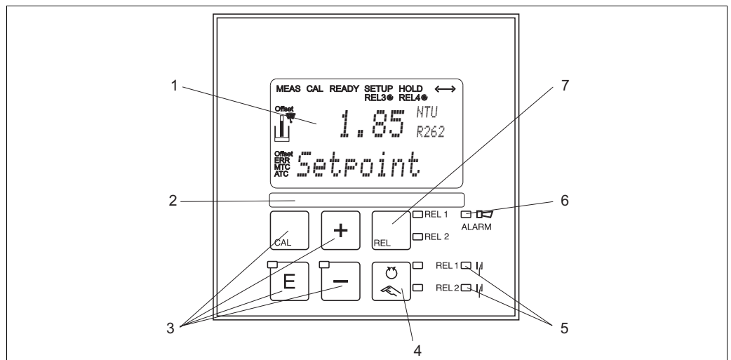
Fig. 15: Operating elements
