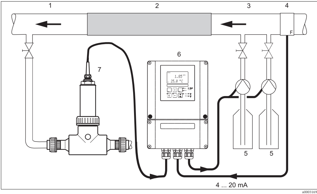
Fig. 21: Arrangement example for feedforward control of the flow rate in the main stream to the PID controller(s) 1 Measuring water extraction point 5 Reagents 2 Static mixer 6 Liquisys M CUM253 3 Injection points 7 CUA250 with CUS31 4 Flowmeter
