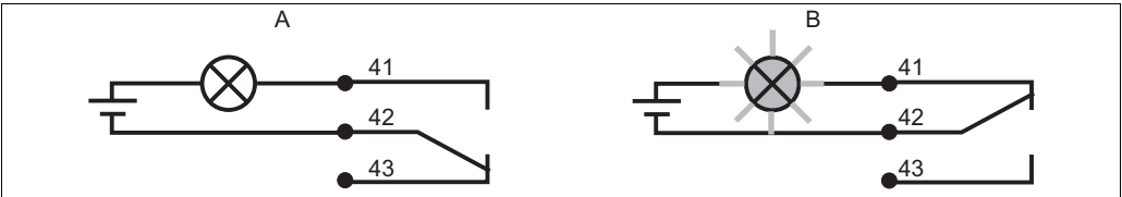
Fig. 13: Recommended fail-safe switching for the alarm contact A Normal operating status B Alarm condition
