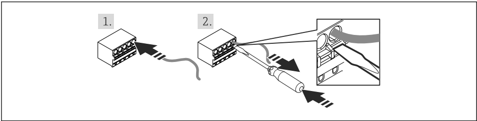
6 Operation of the spring terminals
