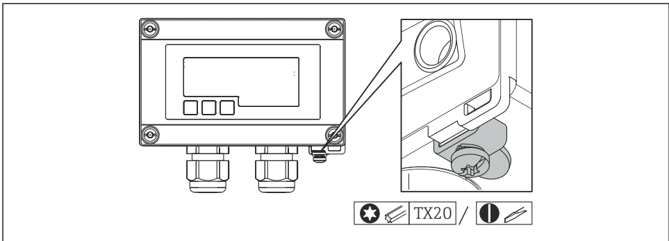
10 Ground terminal on field housing
