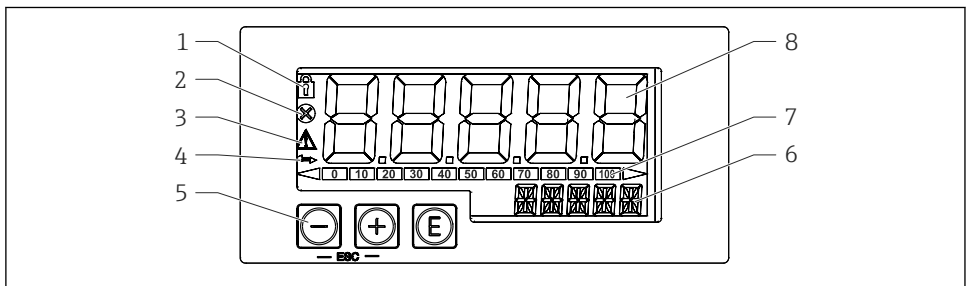
11 Display and operating elements of the process display unit
