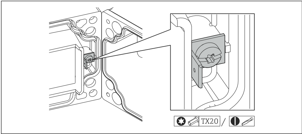
9 Functional grounding terminal in field housing
